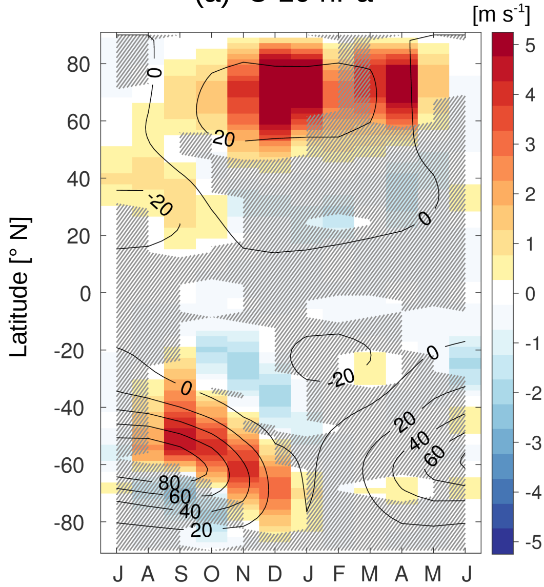
(a) U 10 hPa
