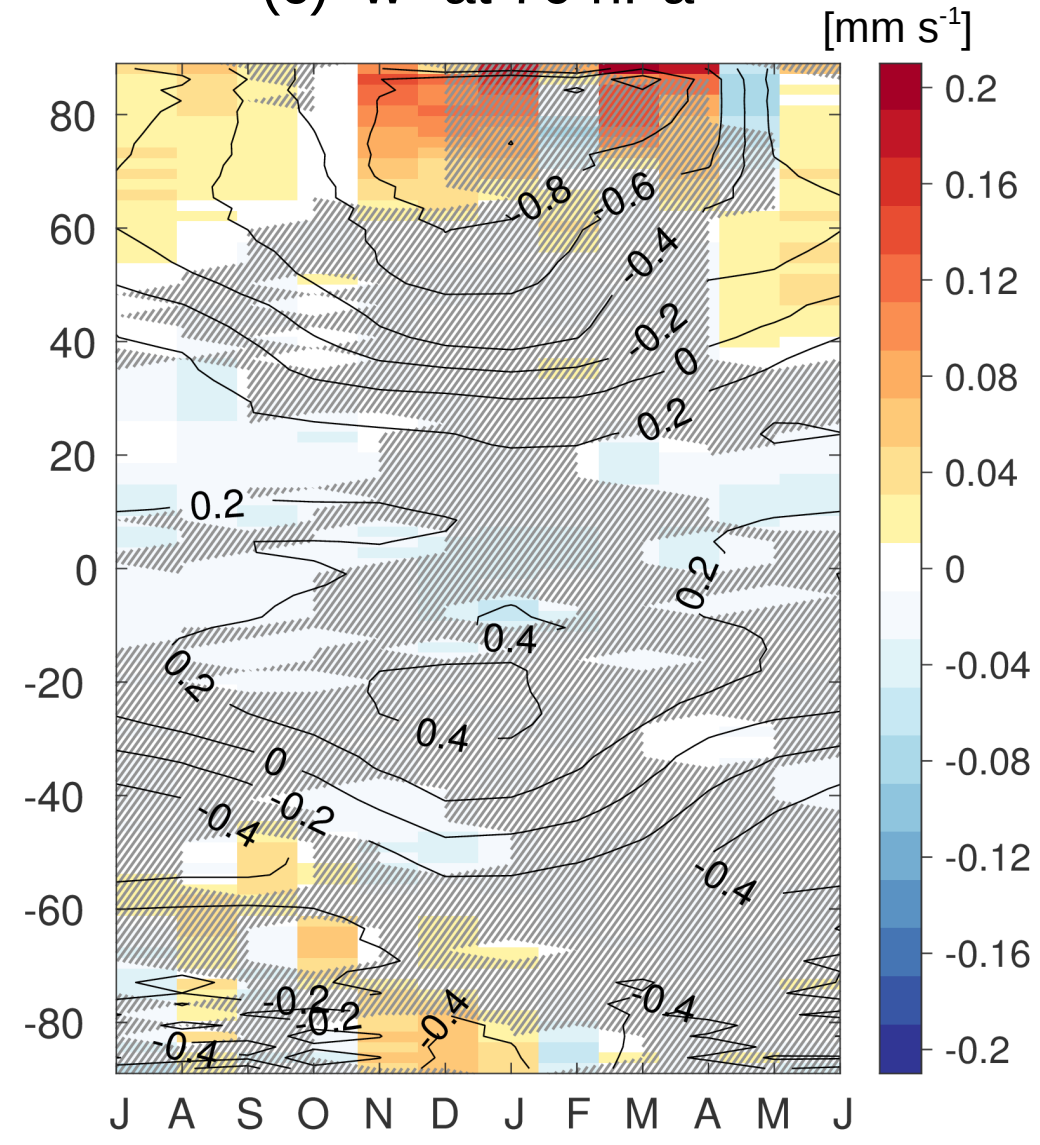
(c) w^* at 70 hPa
