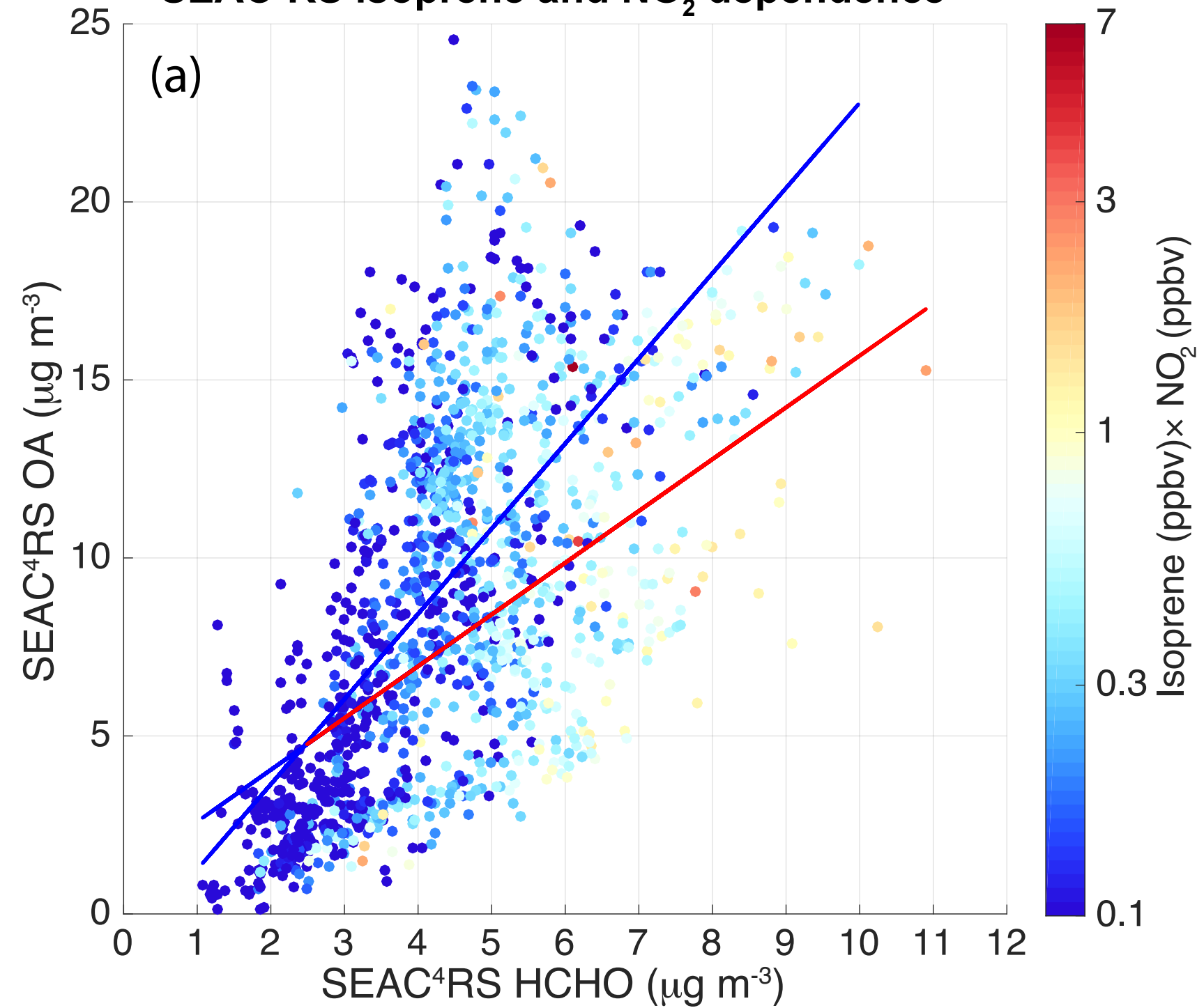
SEAC 4 RS isoprene and NO 2 dependence
