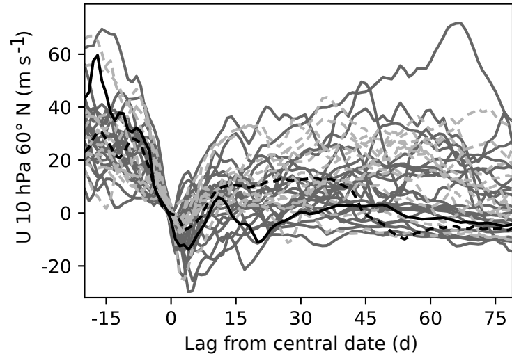
(a) JRA-55 36 events
