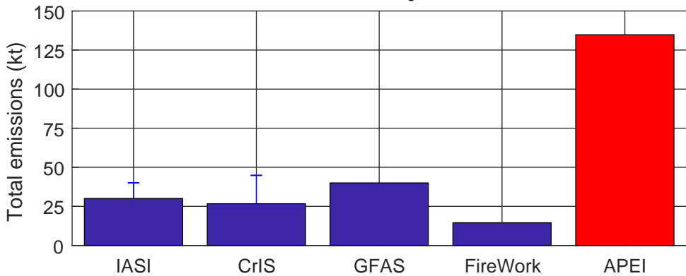
(b) NH 3
