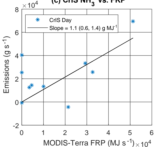
(c) CrIS NH 3 vs. FRP
