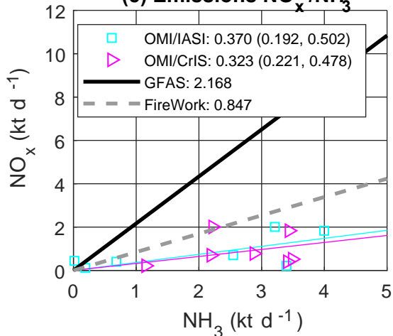
(e) Emissions \text{NO}_x / \text{NH}_3
