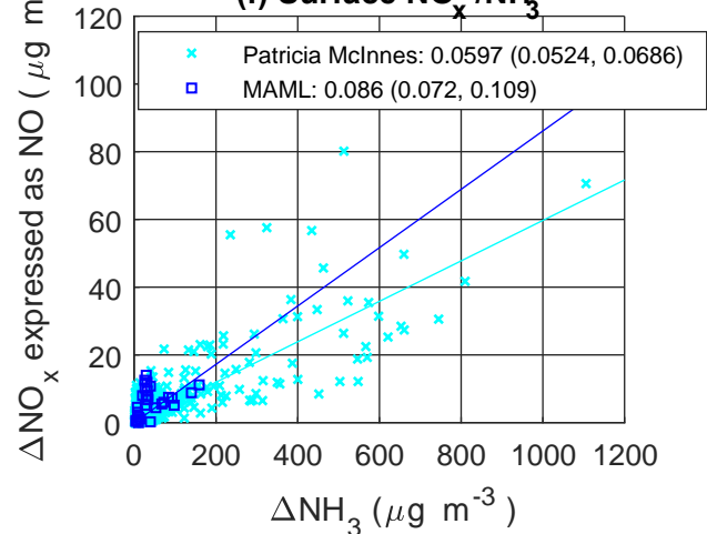
(f) Surface \text{NO}_x / \text{NH}_3
