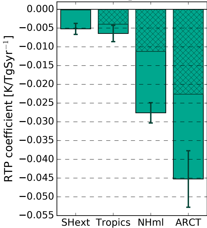
(a) 0xEU SO 2 emissions
