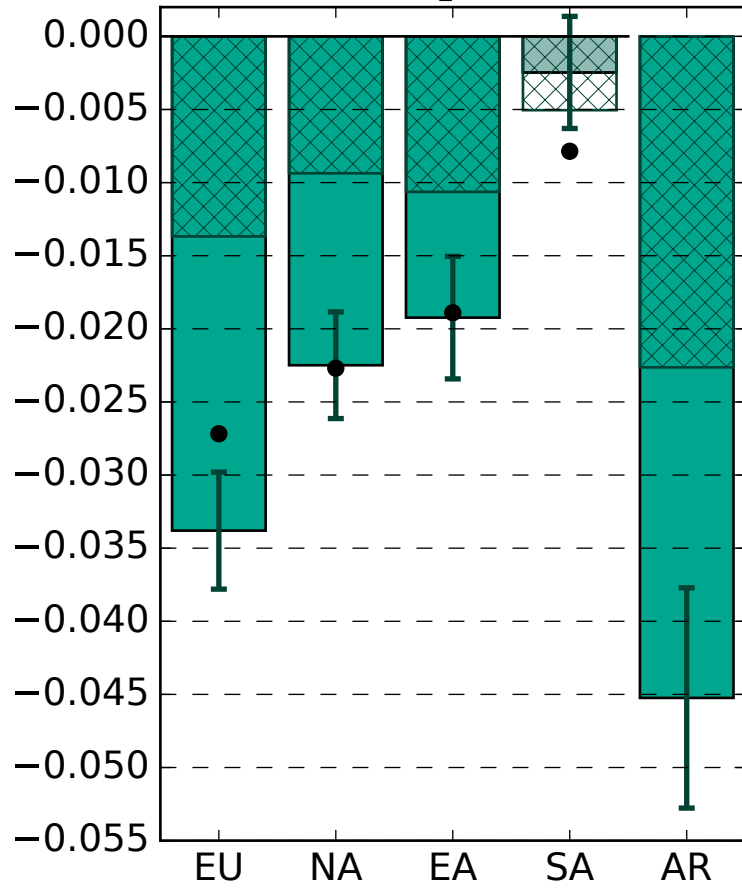
(b) 0xEU SO 2 emissions
