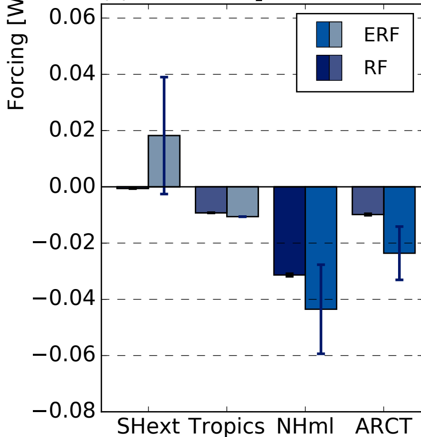
(c) 5xEA SO 2 emissions
