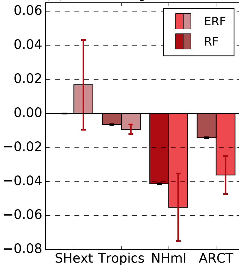
(b) 5xNA SO 2 emissions
