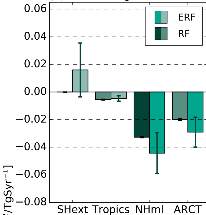
(a) 7xEU SO 2 emissions
