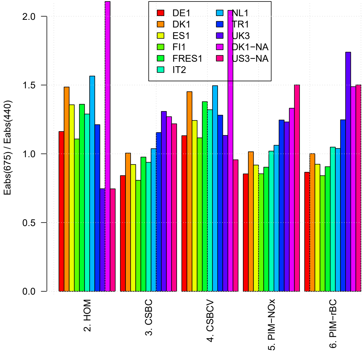
Ratio of Eabs(675) and Eabs(440) at AERONET stations in 2010
