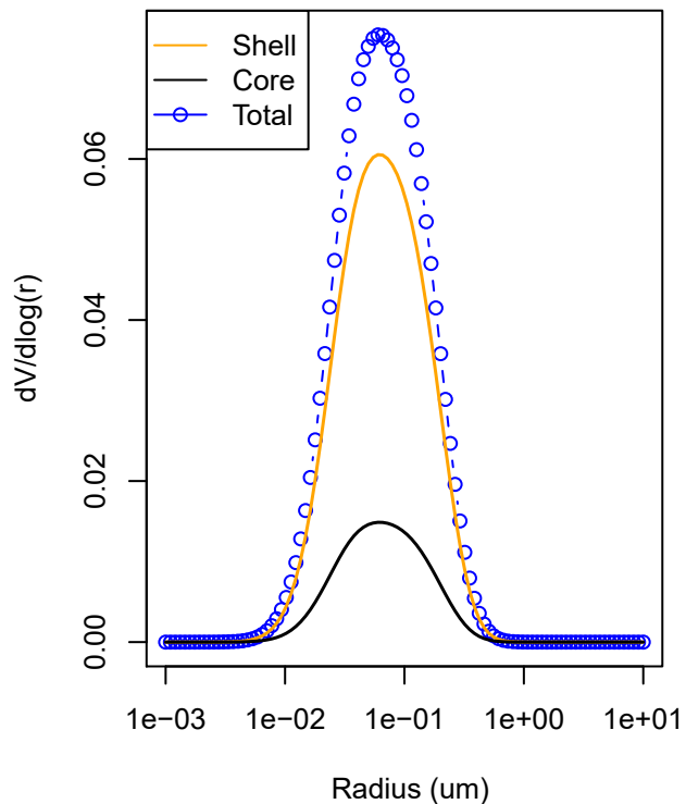
(b) Volume-average log-normals
