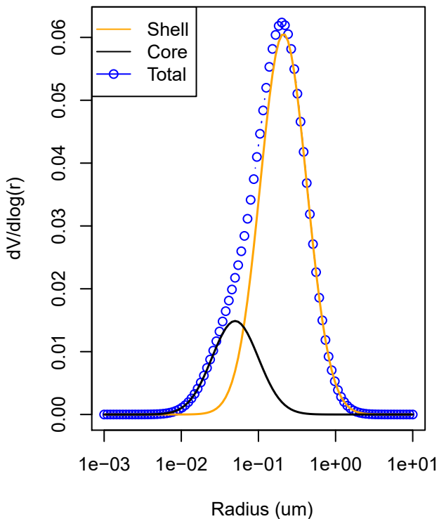
(a) Sum of log-normals
