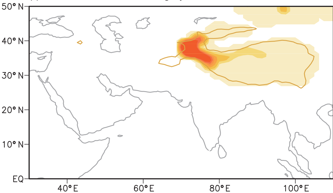
(b) Dust-in-snow surface forcing APR
