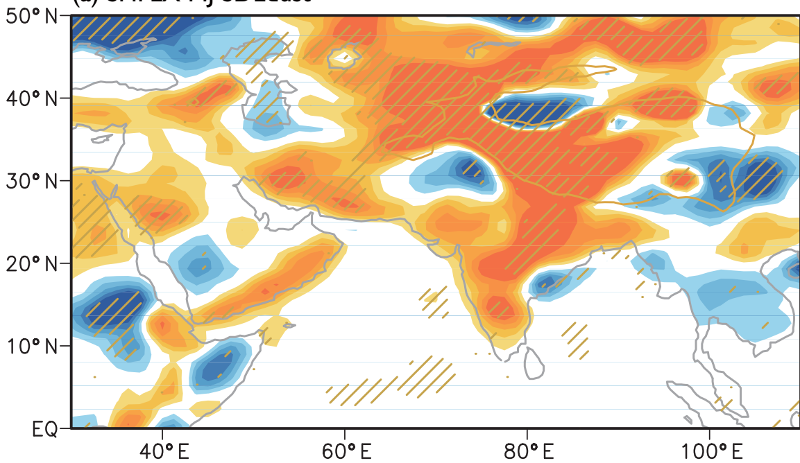
(b) LHFLX MJ SDEdust
