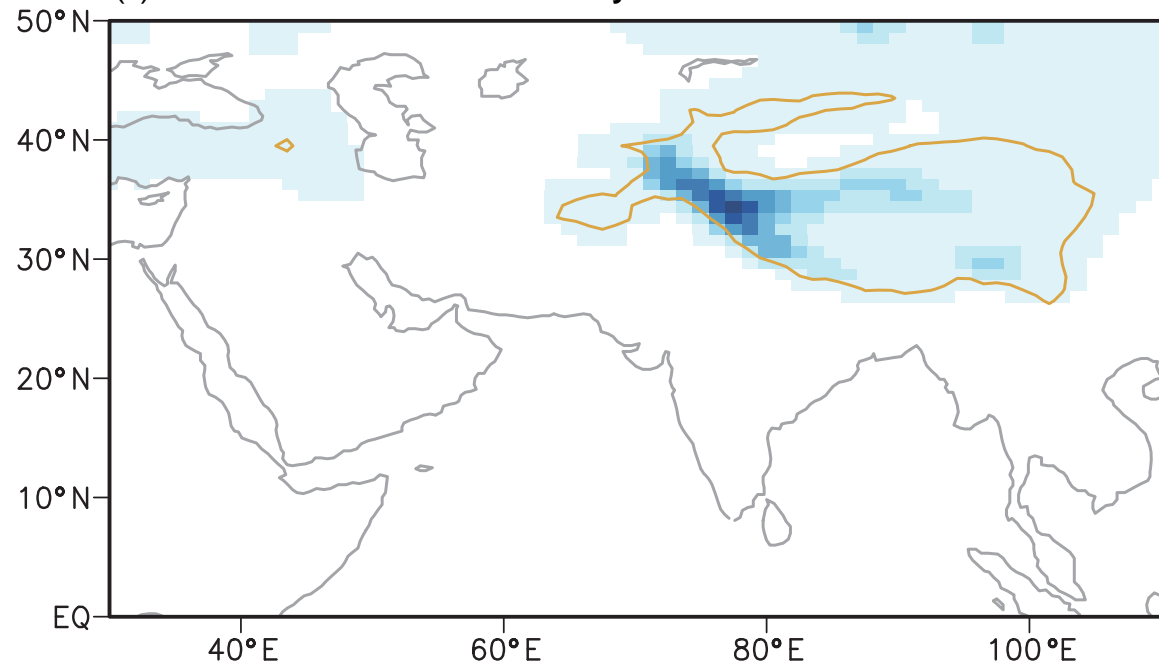
(b) MODIS snow cover fraction MJ
