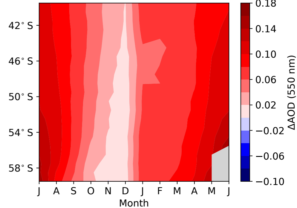
(f) CHEM3-SSF minus MODIS [RMSE=0.081]
