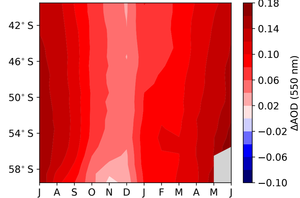
(c) CHEM3 minus MODIS [RMSE=0.105]
