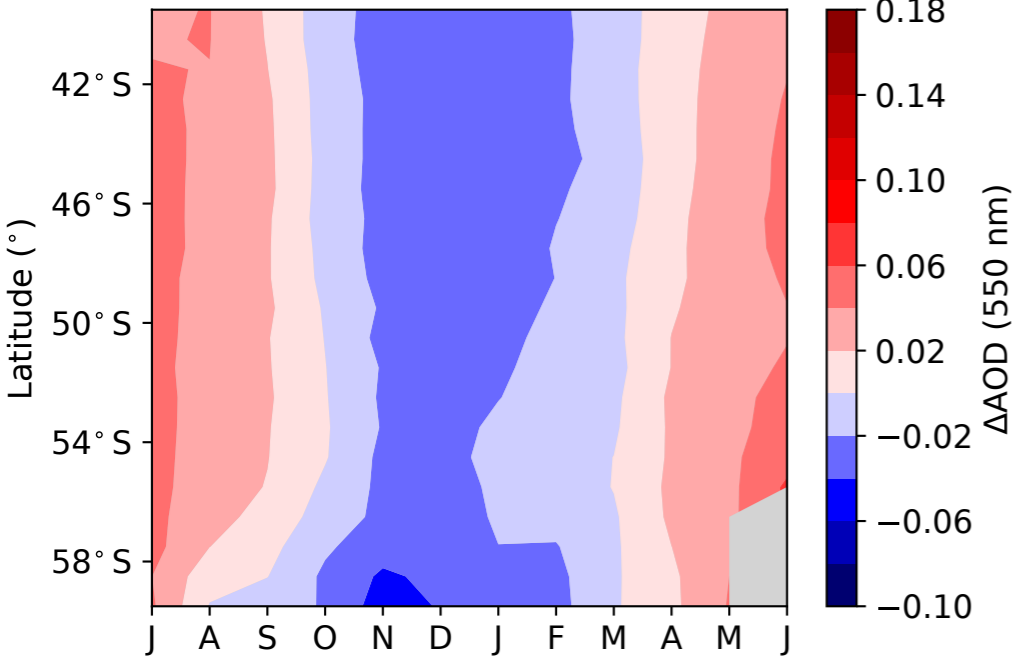
(a) CHEM1 minus MODIS [RMSE=0.028]
