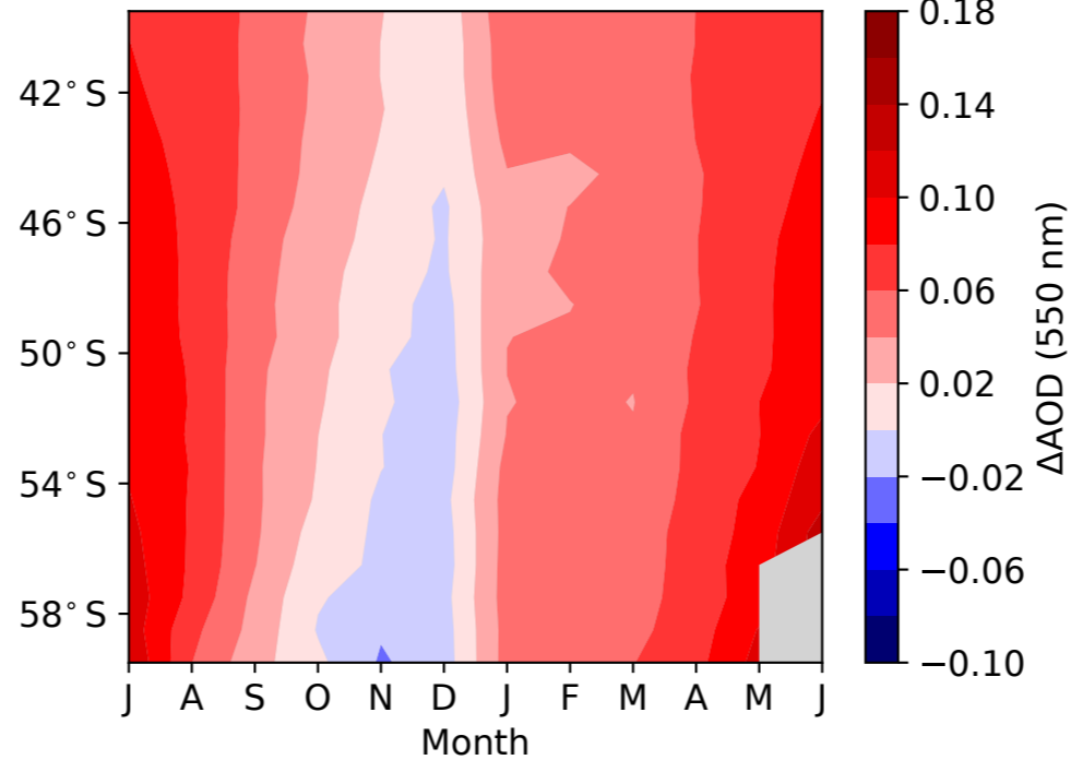
(e) CHEM2-SSF minus MODIS [RMSE=0.059]
