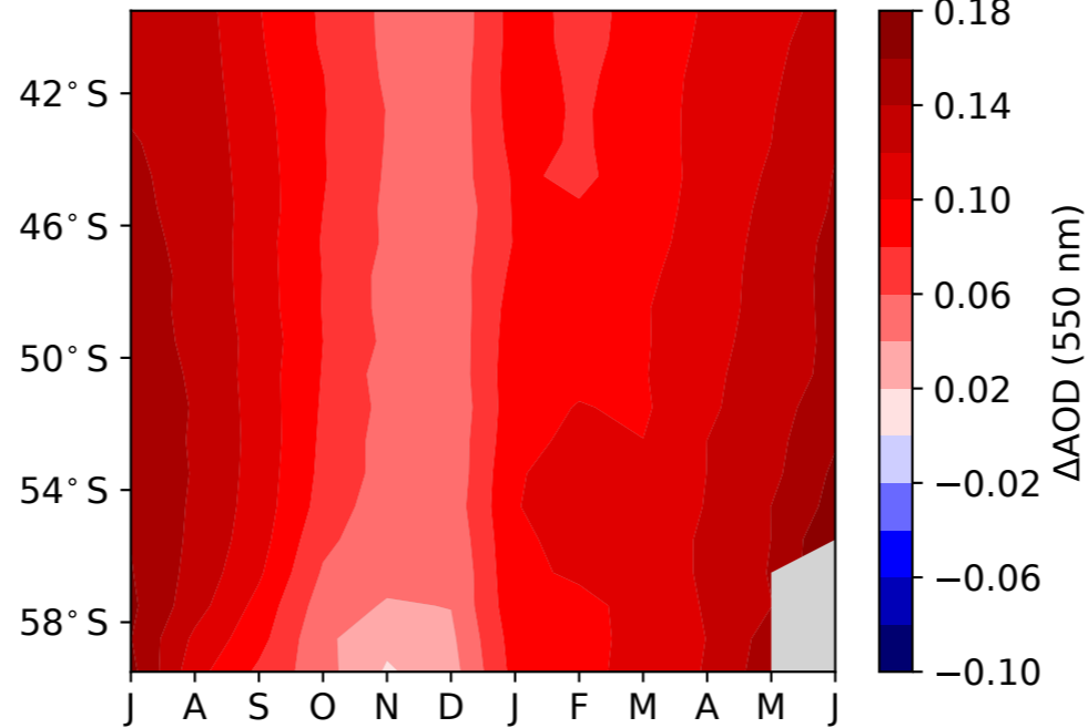
(b) CHEM2 minus MODIS [RMSE=0.107]
