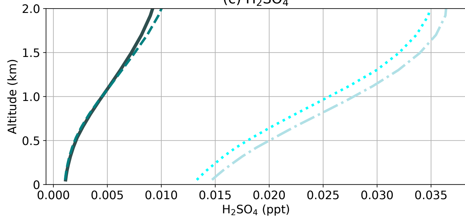
(c) H 2 SO 4
