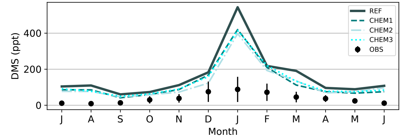
(c) Cape Grim DMS (41°S, 145°E)
