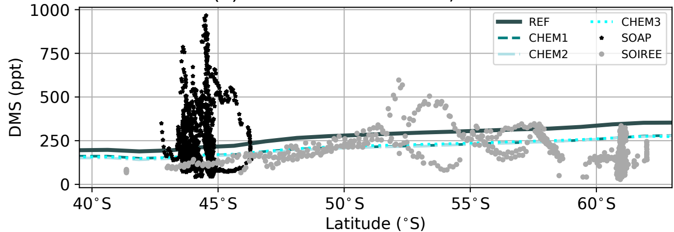
(a) Southern Ocean DMS, Feb-Mar
