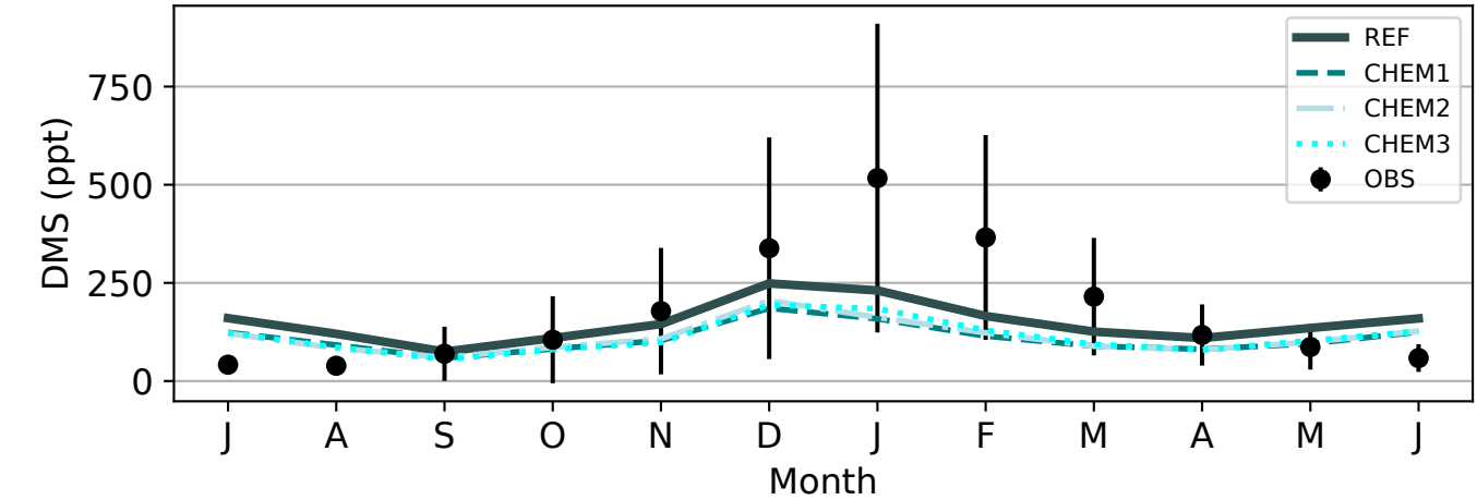
(b) Amsterdam Island DMS (38°S, 78°E)
