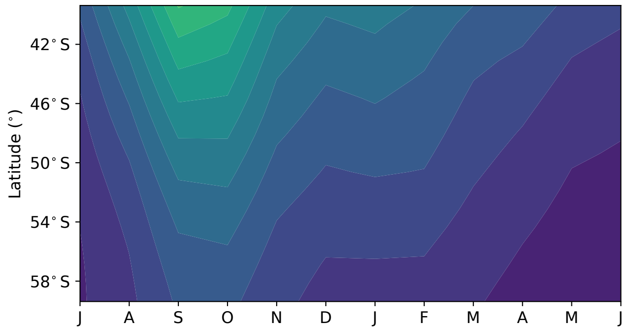
(a) Aitken mode
