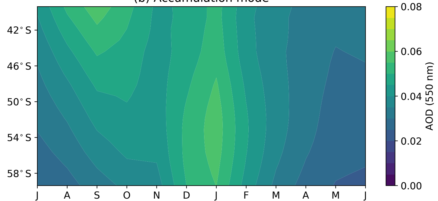
(b) Accumulation mode
