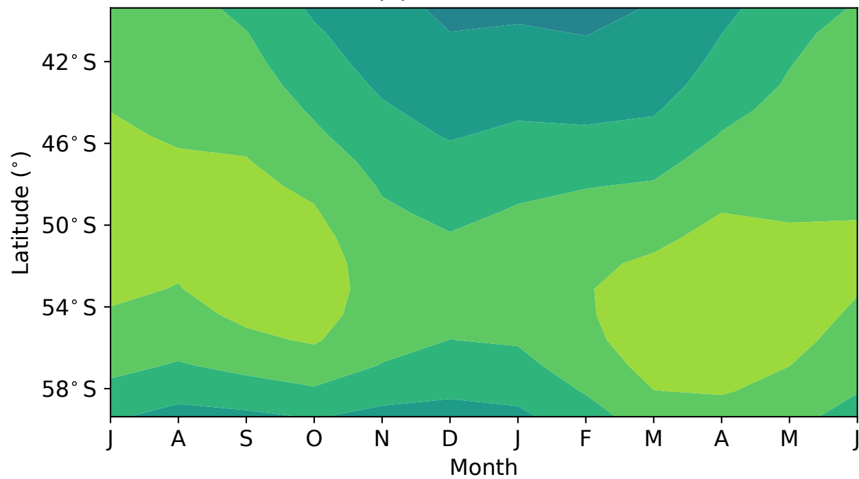
(c) Coarse mode
