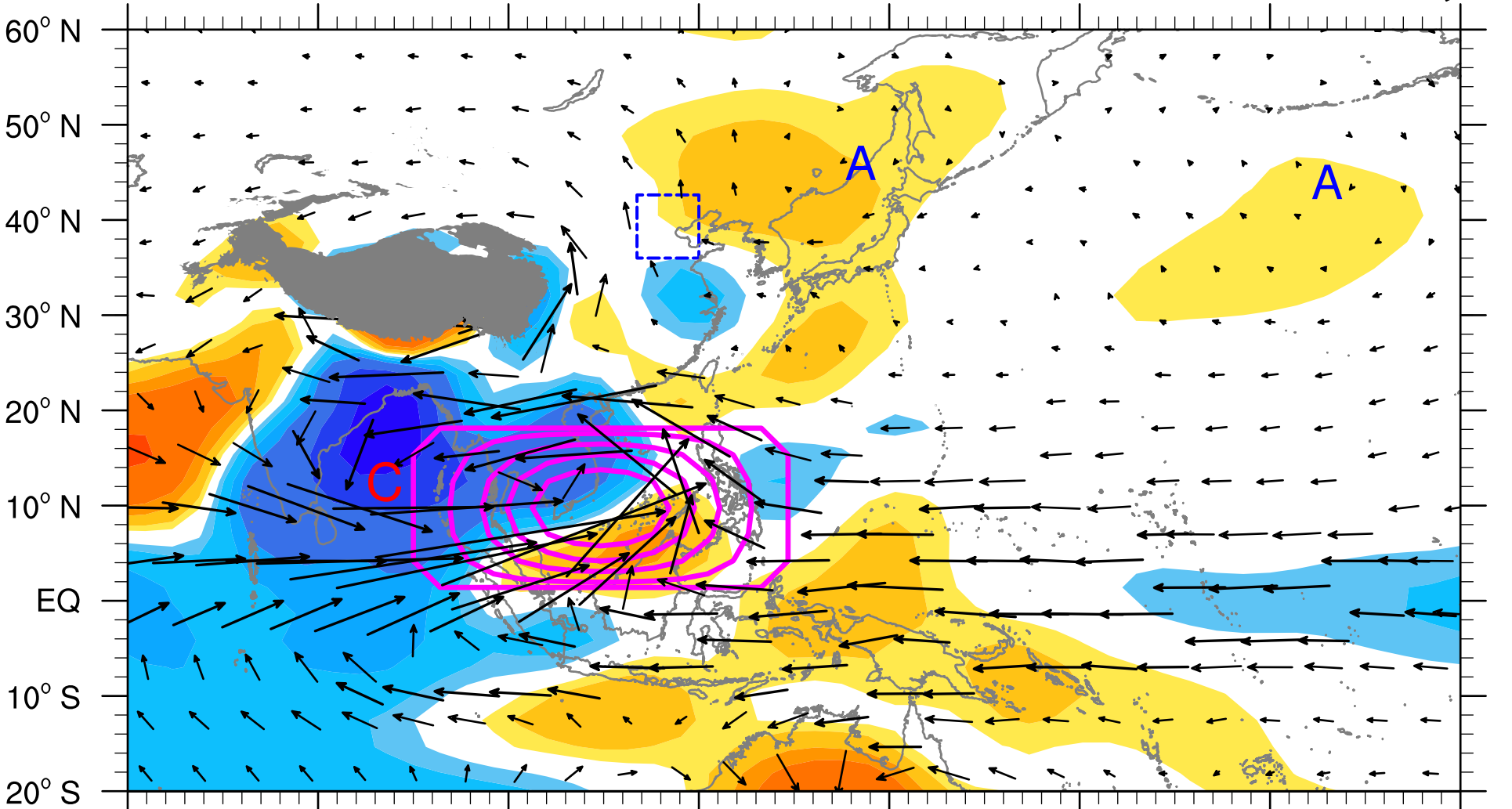
Z850_UV850 response to heating centered at (109.69° E, 9.77° N)
