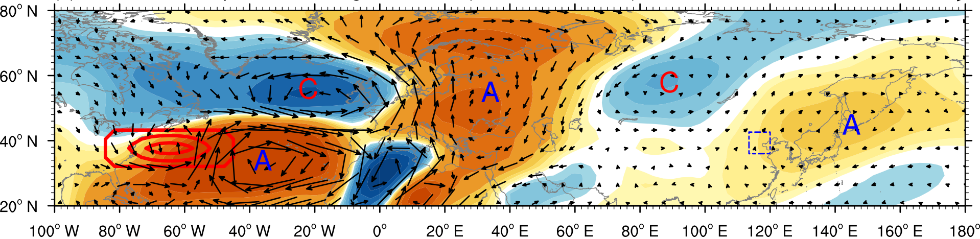
(b) Z500_UV500 response to heating centered at (64.69° W, 37.67° N)
