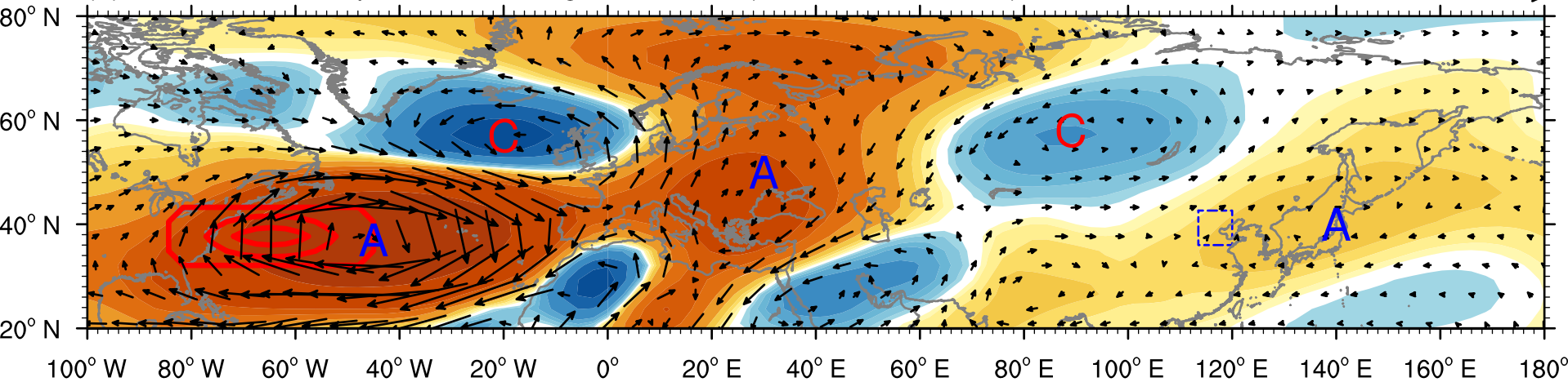
(a) Z200_UV200 response to heating centered at (64.69° W, 37.67° N)
