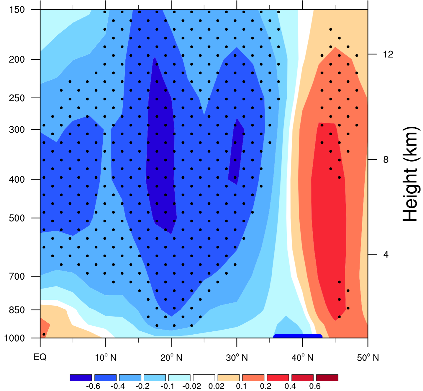
(a) SON omega reg. onto SST over R2 (y-p profile, 112.5°–130° E)
