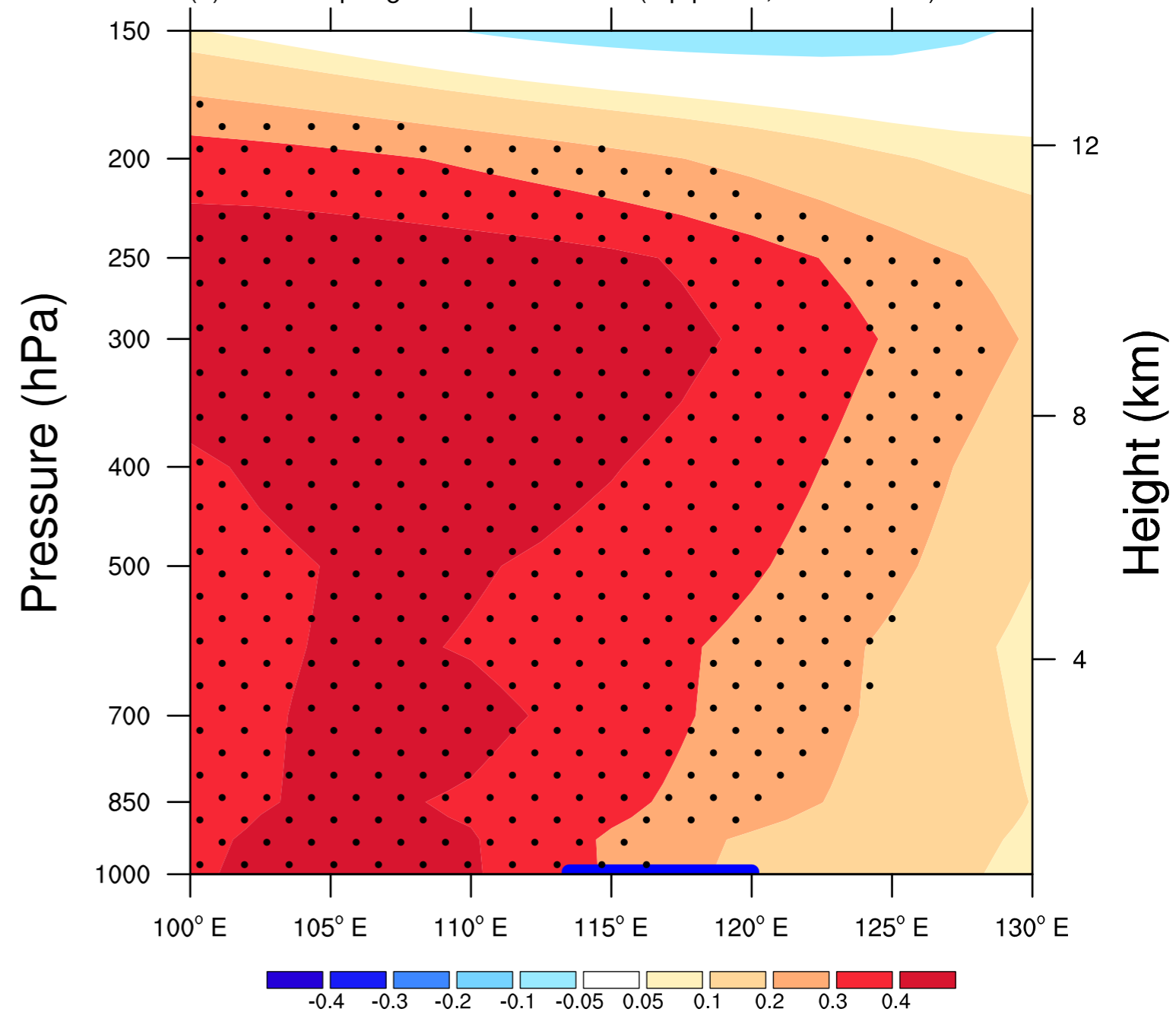
(b) SON temp reg. onto SST over R2 (x-p profile, 35°–42.5° N)
