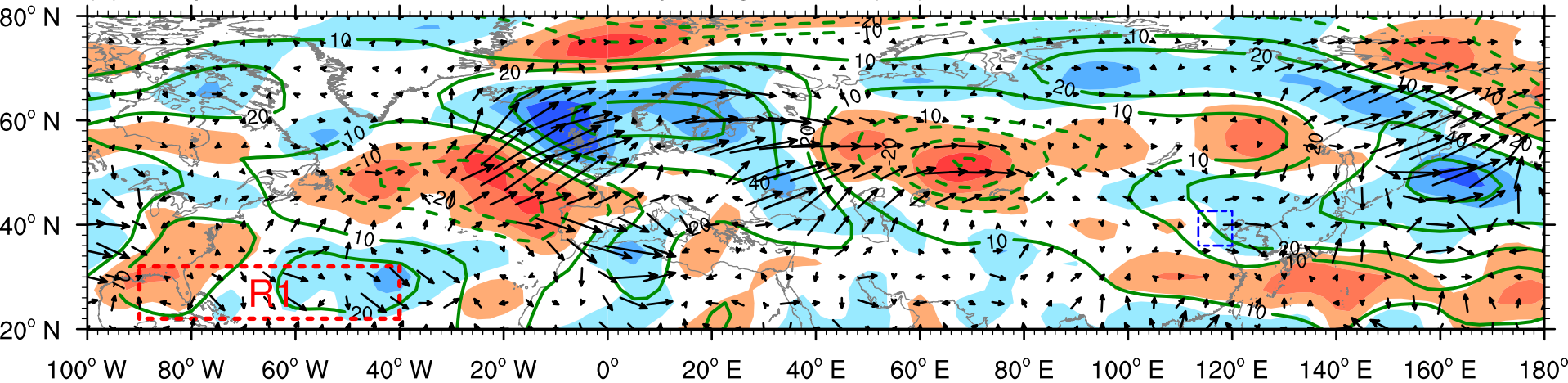
(b) Composite diff. of SON 500 hPa Vorticity_Height_WAF (R1)
