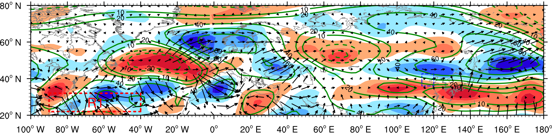
(a) Composite diff. of SON 200 hPa Vorticity_Height_WAF (R1)
