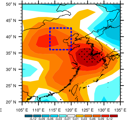
(f) SON OMEGA500 reg. onto AHD_{BTH}
