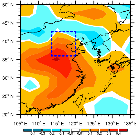
(a) SON surface RH reg. onto AHD_{BTH}
