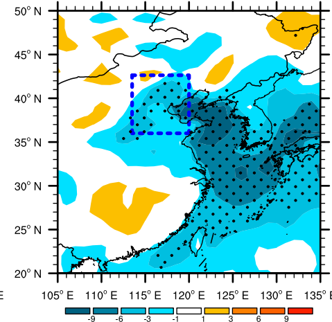
(e) SON PBLH reg. onto AHD_{BTH}
