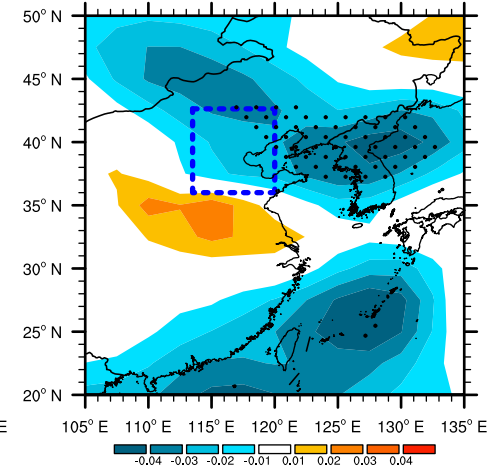
(c) SON surface wind reg. onto AHD_{BTH}
