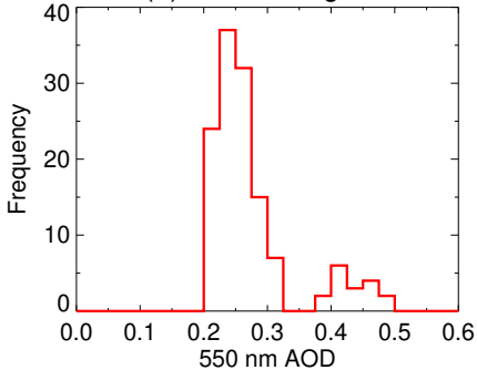
(b) AOD histogram
