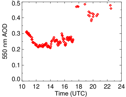
(a) AERONET AOD on 5 July 2011
