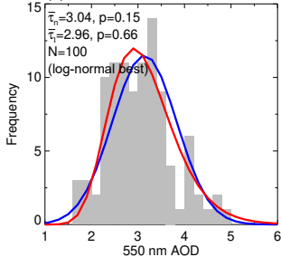
(c) Pontianak, 21 October 2015
