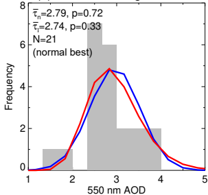
(b) Moscow, 6 August 2010
