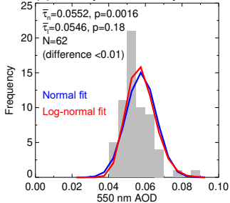
(a) Midway Island, 3 July 2006
