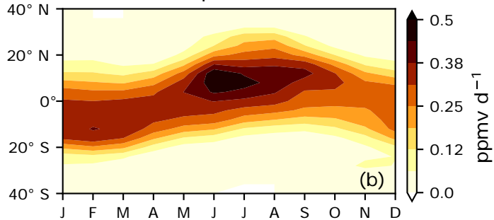
Ice evaporation rate
