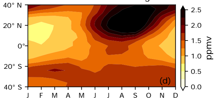
Convective moistening
