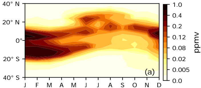
GEOSCCM convective ice
