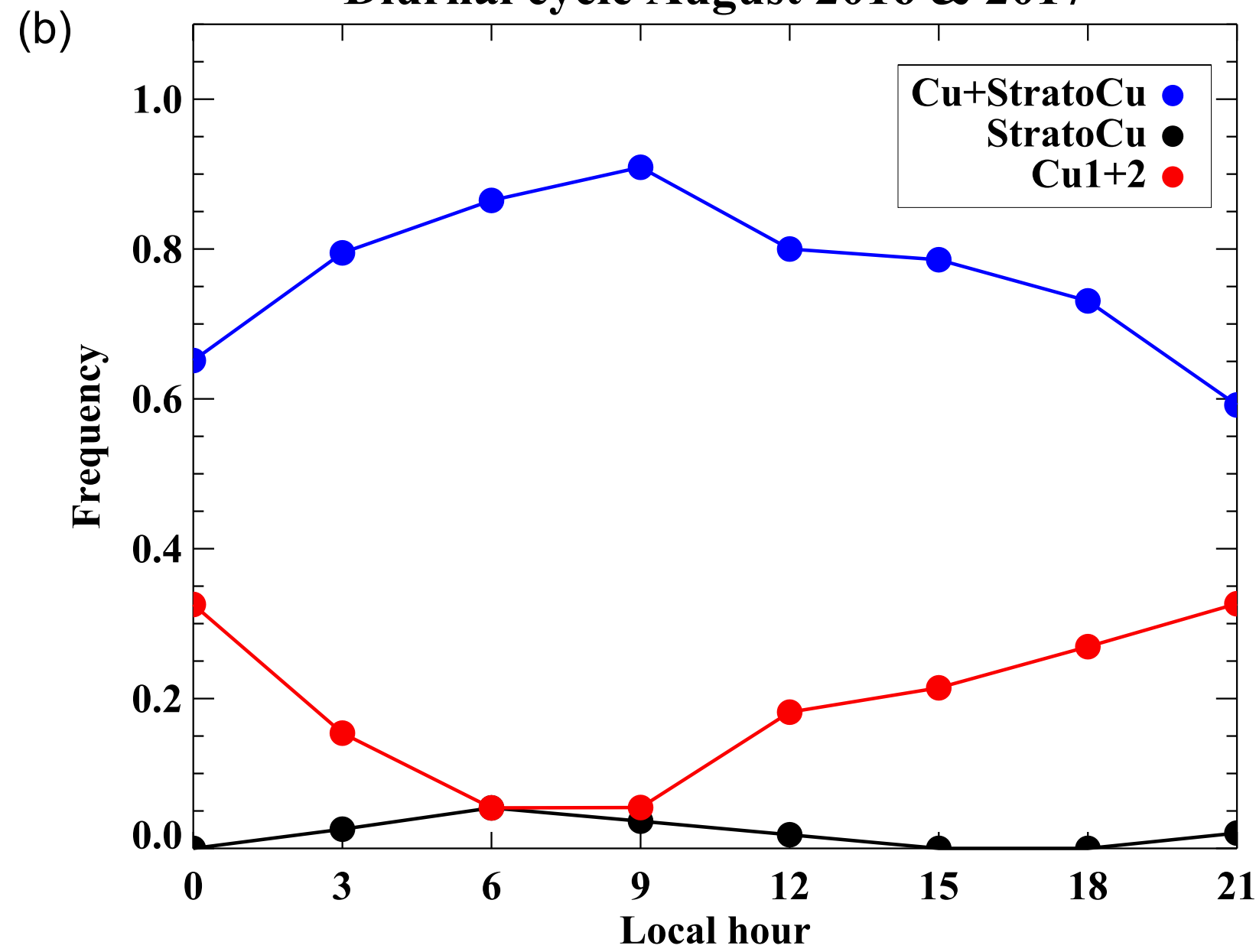
Diurnal cycle August 2016 & 2017
