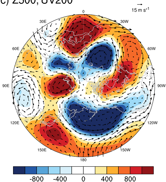
(c) Z500, UV200
