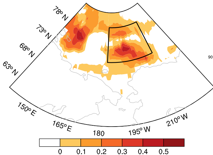
(c) Z500, UV200
