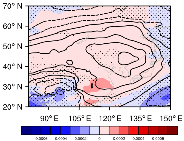
(c) Shum850,Z500| Dec-Jan
