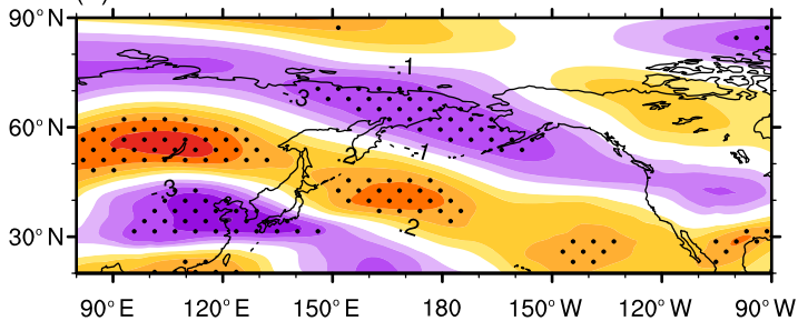
(c) Z850,UV
