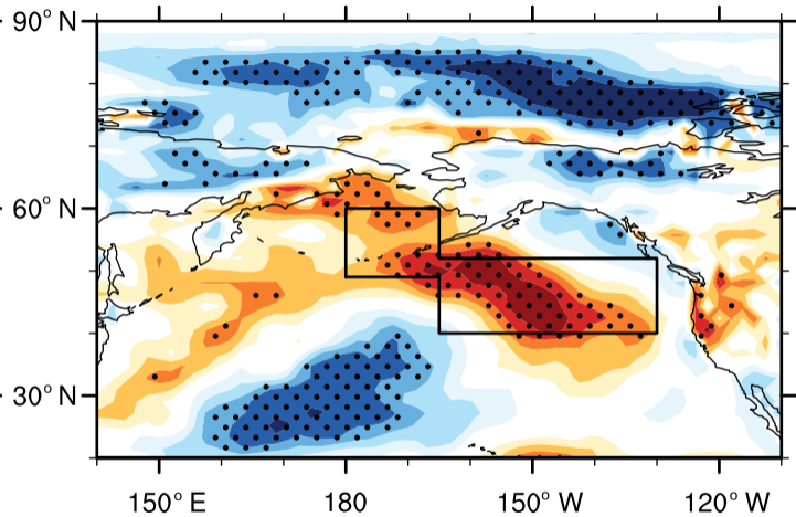
(b) Latent heat flux
