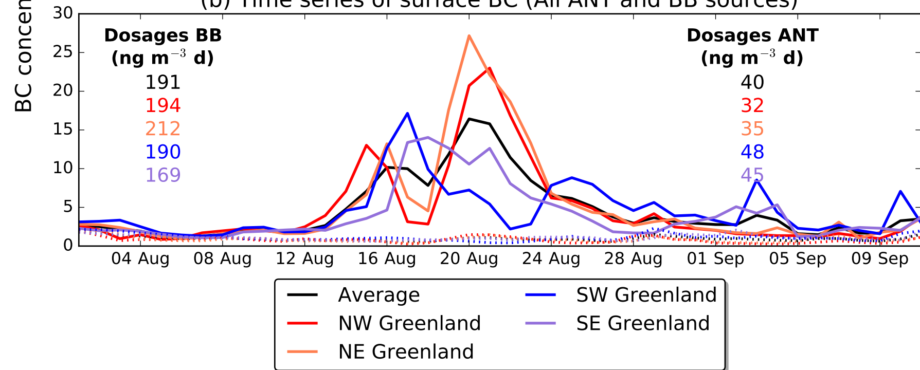
(b) Time series of surface BC (All ANT and BB sources)
