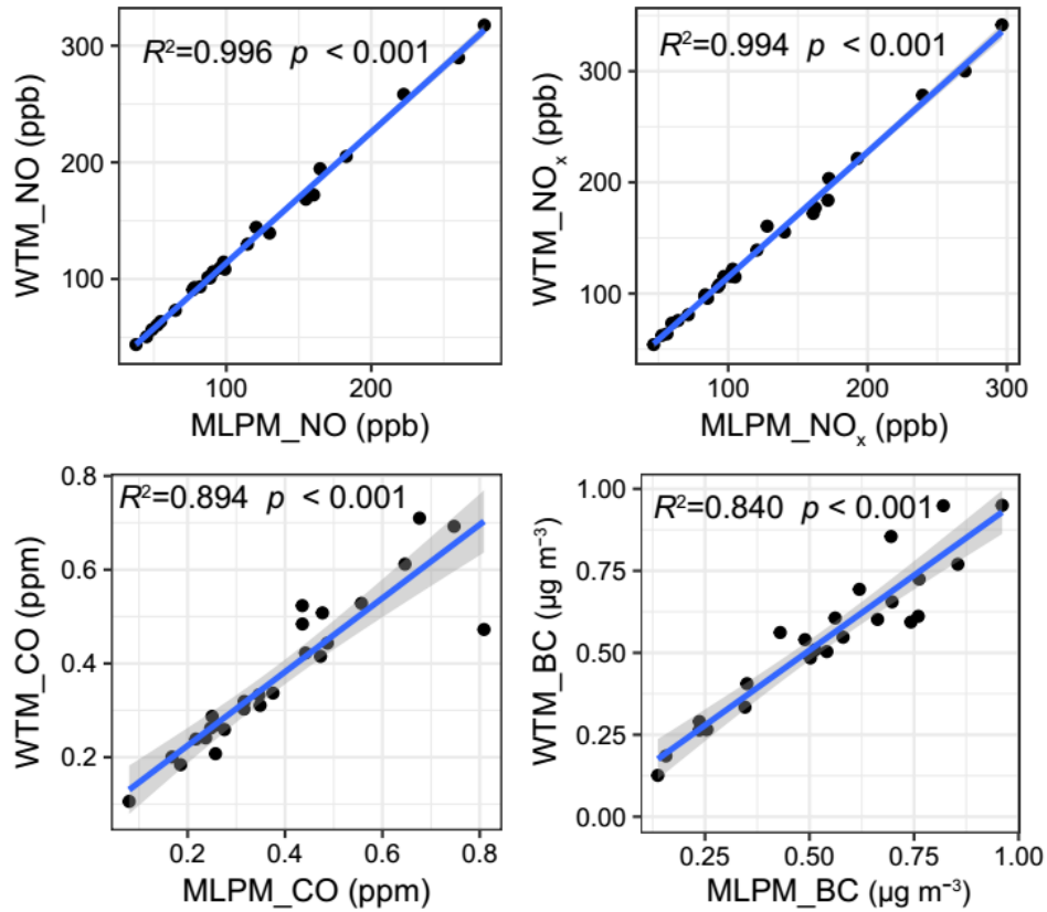
Figure S4. Correlations between the on-road emission concentrations (i.e. C_{veh.} ) obtained by the wavelet transform method (WTM) and the moving low percentile method (MLPM) in each day for NO, NO x , BC, CO, SO 2 , and O 3 . The blue line shows the linear fit curve and the gray area is the 95% confidence interval.
