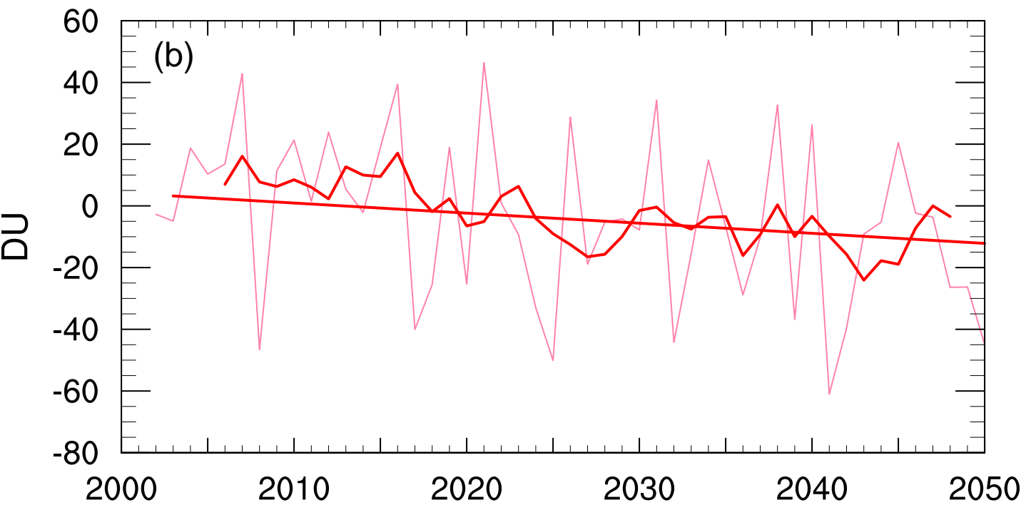
\Delta PCO (SEN-REF), LS, Antarctic, September
