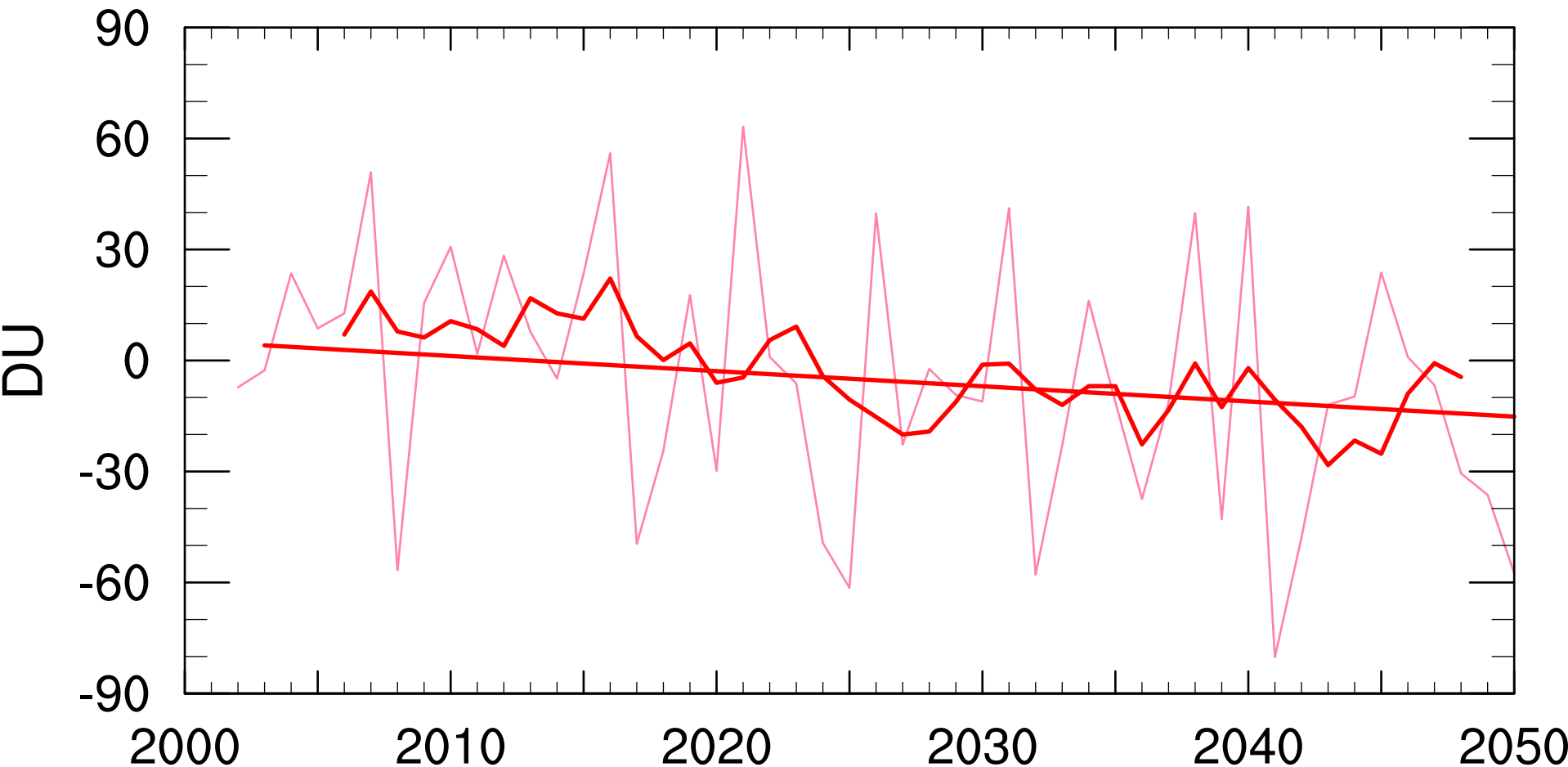
\Delta TCO (SEN-REF), Antarctic, September
