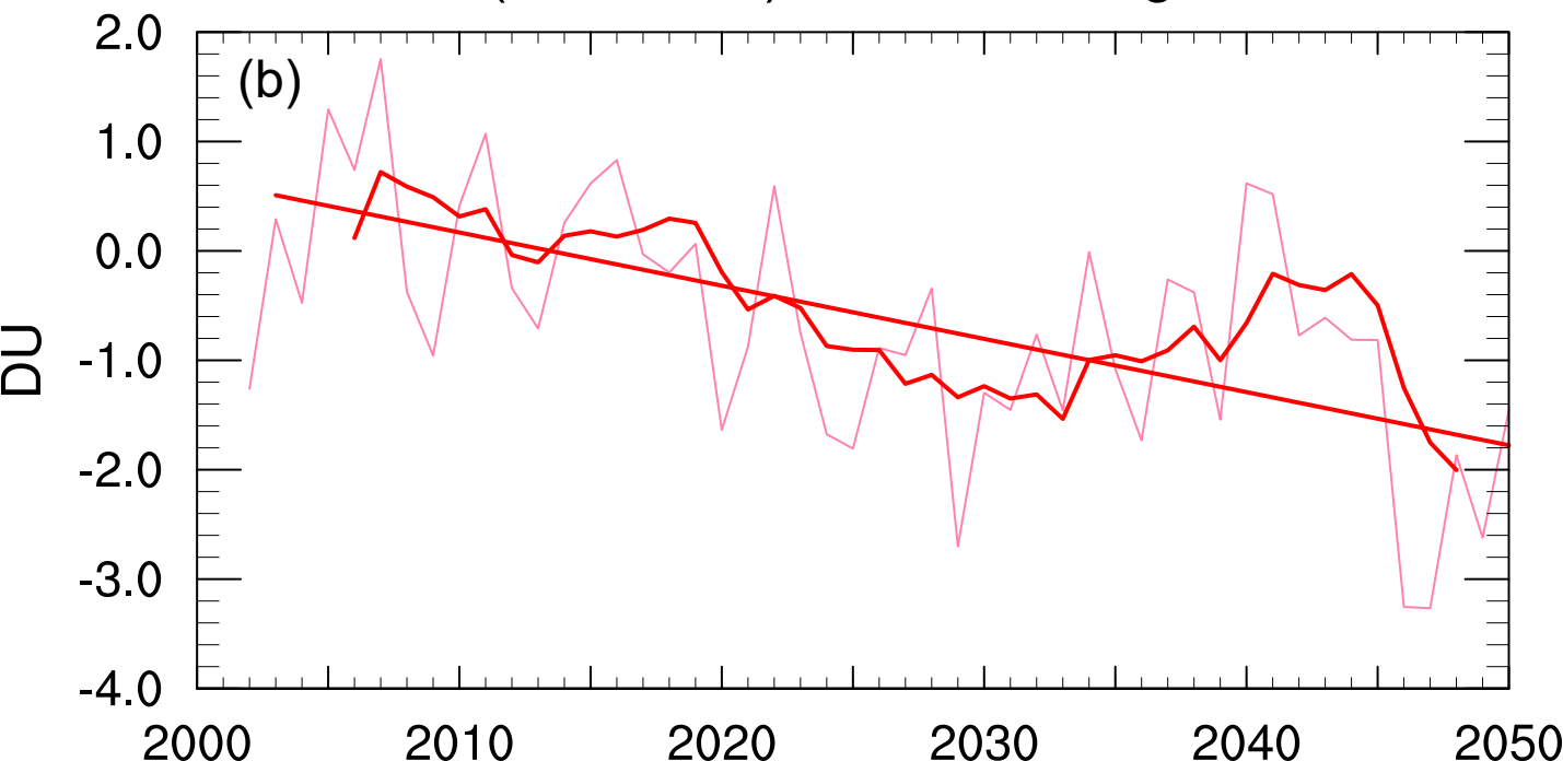
\Delta TCO (SEN-REF), annual near-global mean
