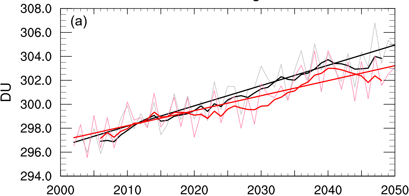
TCO, annual near-global mean
