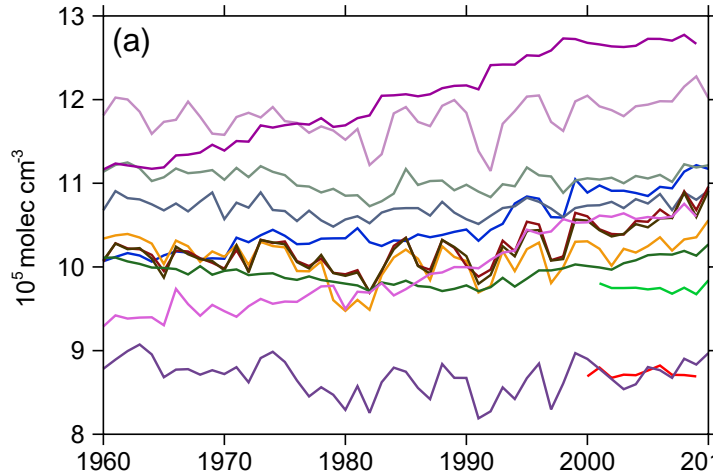
Global tropospheric OH
