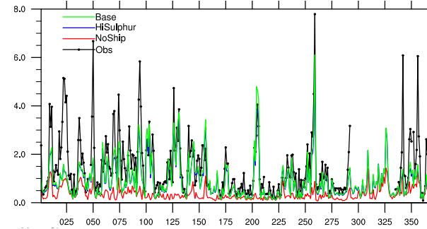
(f) Anholt NO 2 concentrations in \mu\text{g(N)}\text{m}^{-3}
