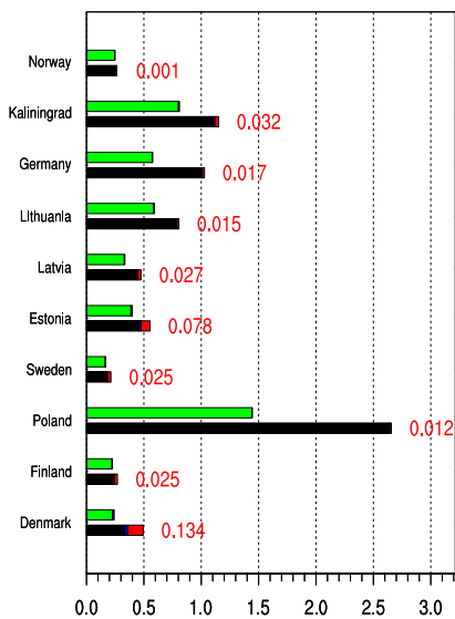
(a) SO 2 in µgS m -3
