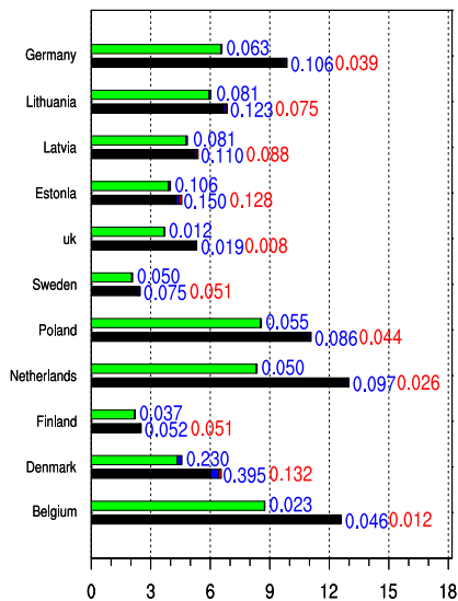
(c) PM 2.5 in µg m -3
