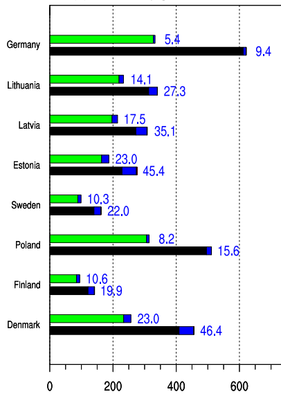
(e) Dep. oxidised nitrogen in mgN m -2
