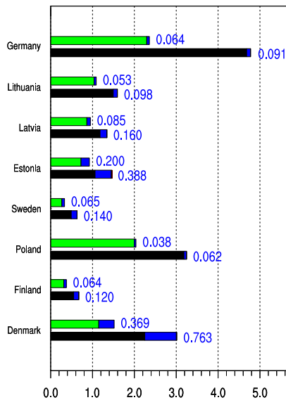
(b) NO 2 in µgN m -3
