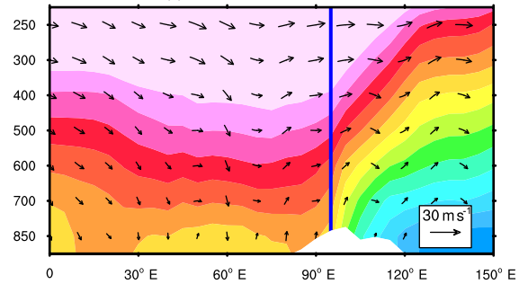
(g) Autumn, 40–60° N
