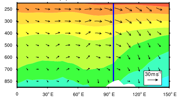
(h) Winter, 40–60° N
