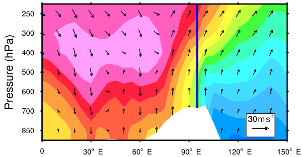
(c) Autumn, 20–40° N
