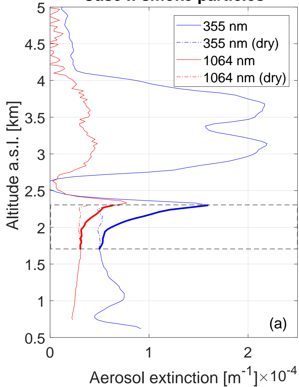
Case I: smoke particles
