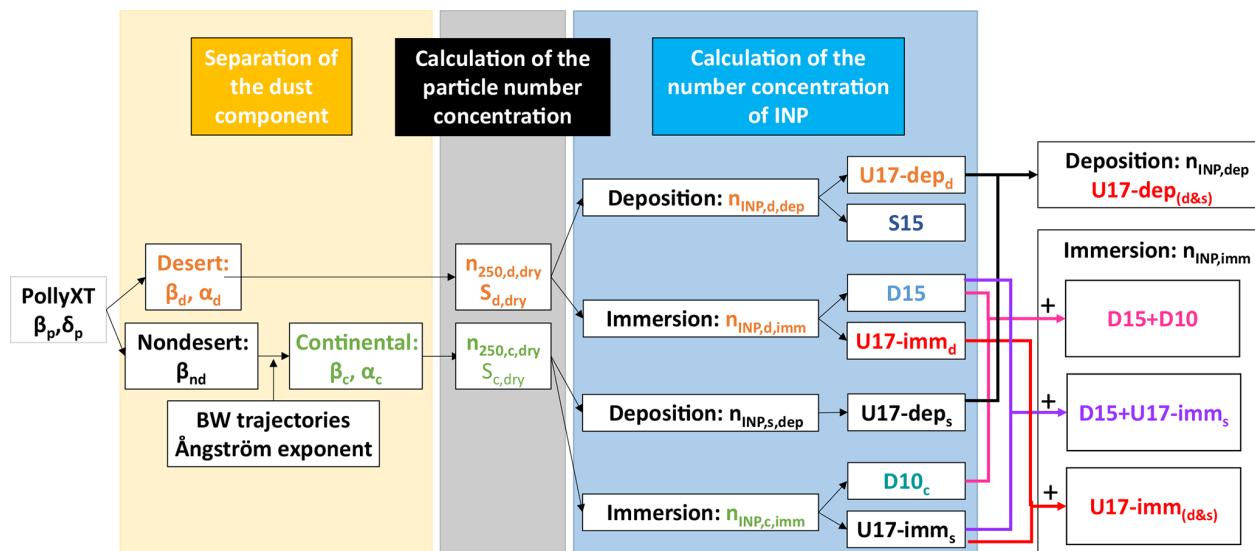
Figure A1. Overview of the data analysis scheme followed for the PollyXT measurements in this work. In the first step, we separate desert and non-desert backscatter coefficients ( \beta_d and \beta_{nd} ) by means of the particle linear depolarization ratio ( \delta_p ). The backscatter coefficients for the non-desert aerosol are estimated to be continental aerosol mixtures \beta_c by means of, e.g., backward (BW) trajectory analysis and Ångström exponent information. The two backscatter coefficients are then converted to aerosol type-dependent particle extinction coefficients ( \alpha_i ). In the next step, the extinction coefficients are converted to aerosol type-dependent profiles of particle number concentrations ( n_{250,i,dry} ) and particle surface area concentration ( S_{i,dry} ). In the next step, ice-nucleating particle number concentrations ( n_{\text{INP},i} ) are estimated by applying INP parameterizations from the literature indicated by D10, D15, S15 and U17 for DeMott et al. (2010, 2015), Steinke et al. (2015) and Ullrich et al. (2017), respectively. Finally, the INP concentrations estimated for the different aerosol types are summed in order to estimate the total n_{\text{INP}} .
