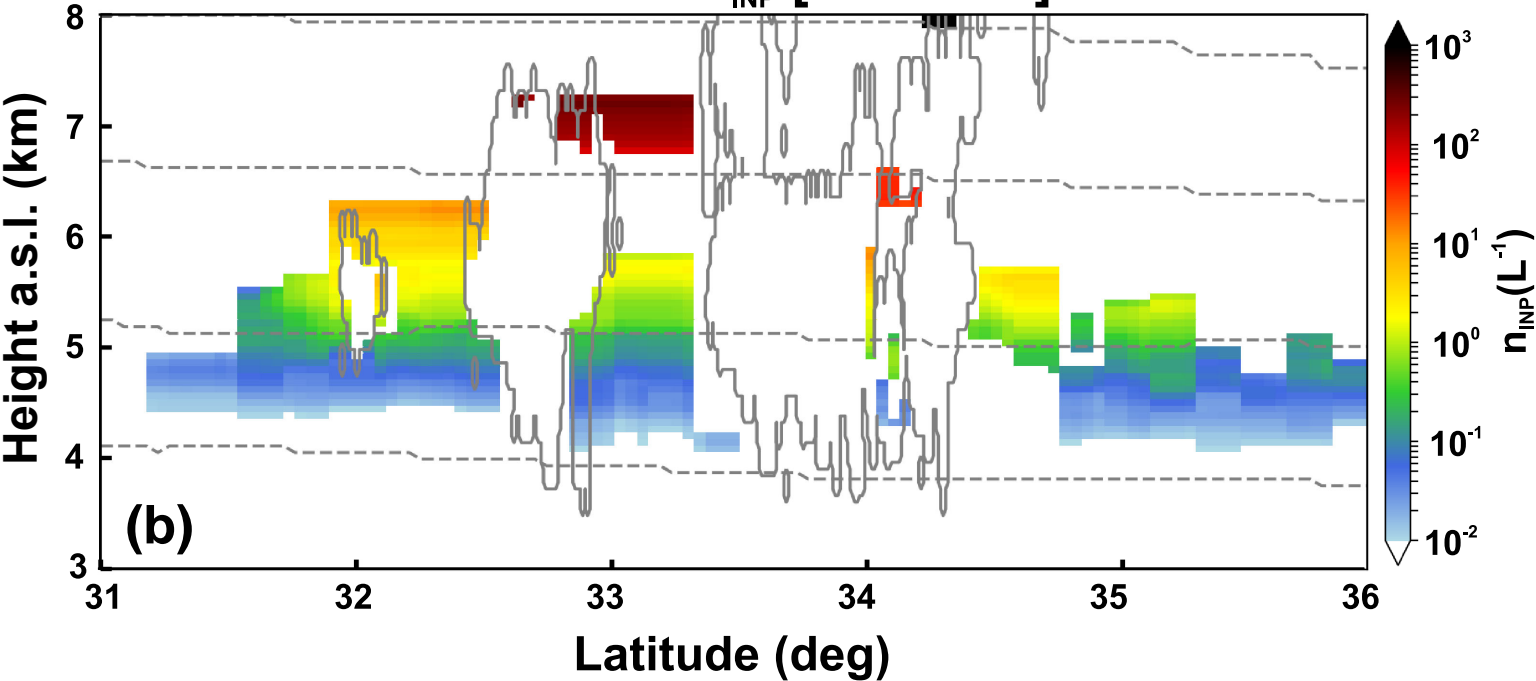
CALIPSO - n_{\text{INP}} [U17-imm]
