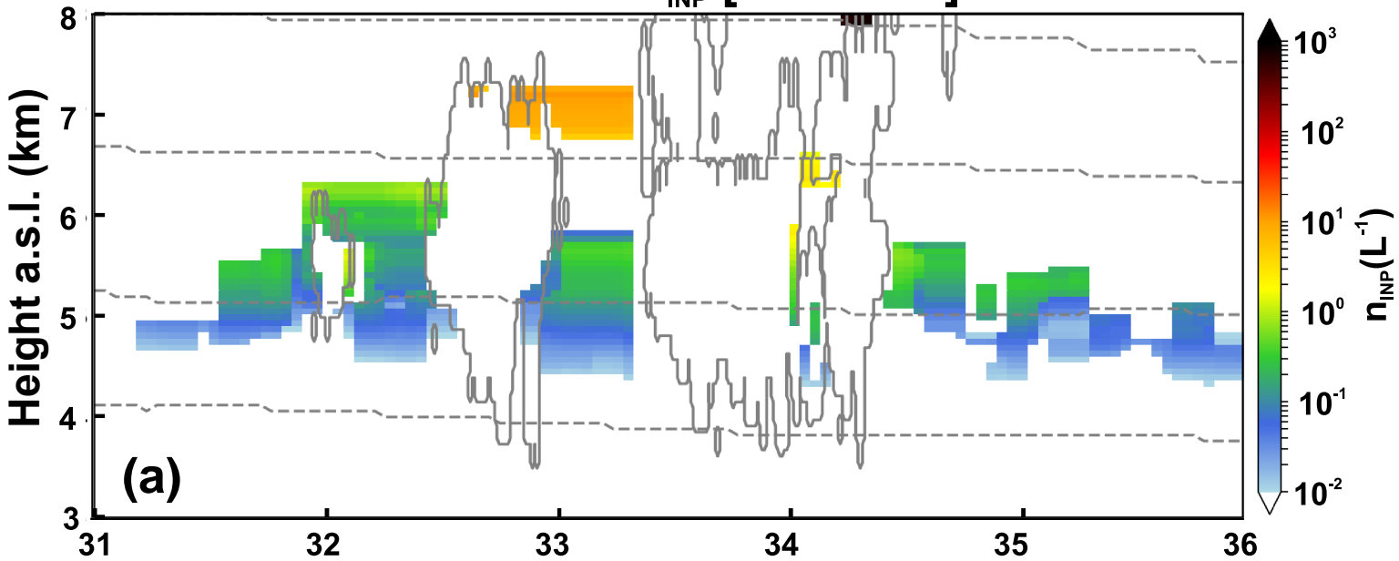
CALIPSO - n_{\text{INP}} [U17-imm]
