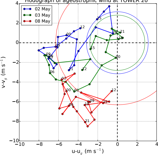
Hodograph of ageostrophic wind at TOWER 20
