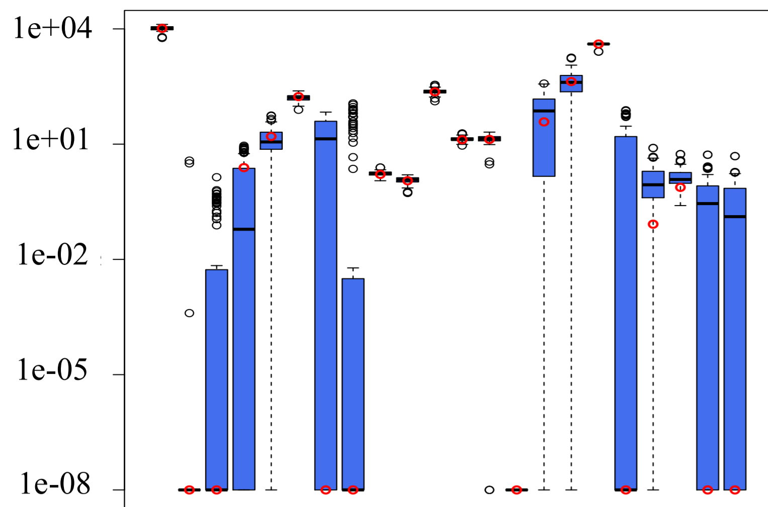
Nitrate [ng m -3 ]
