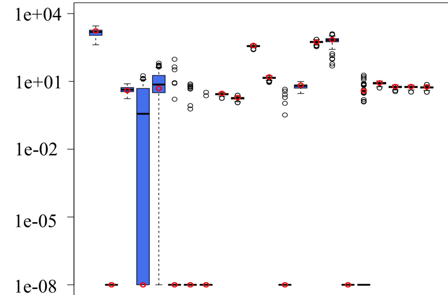
Traffic [ng m -3 ]
