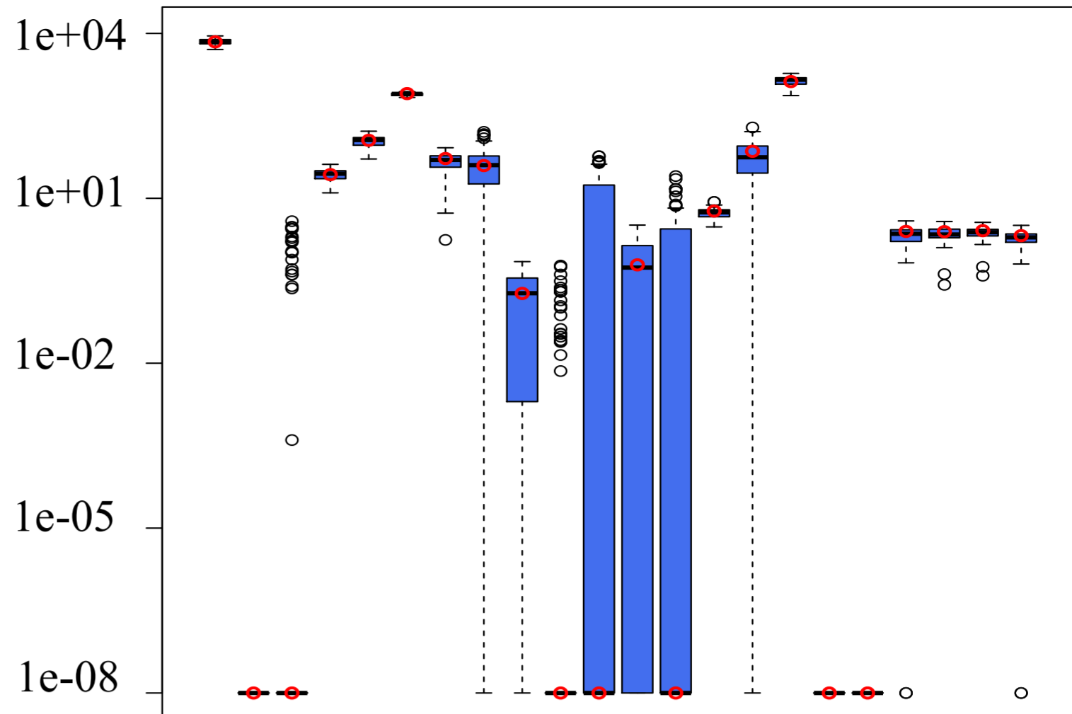
Sulfate [ng m -3 ]
