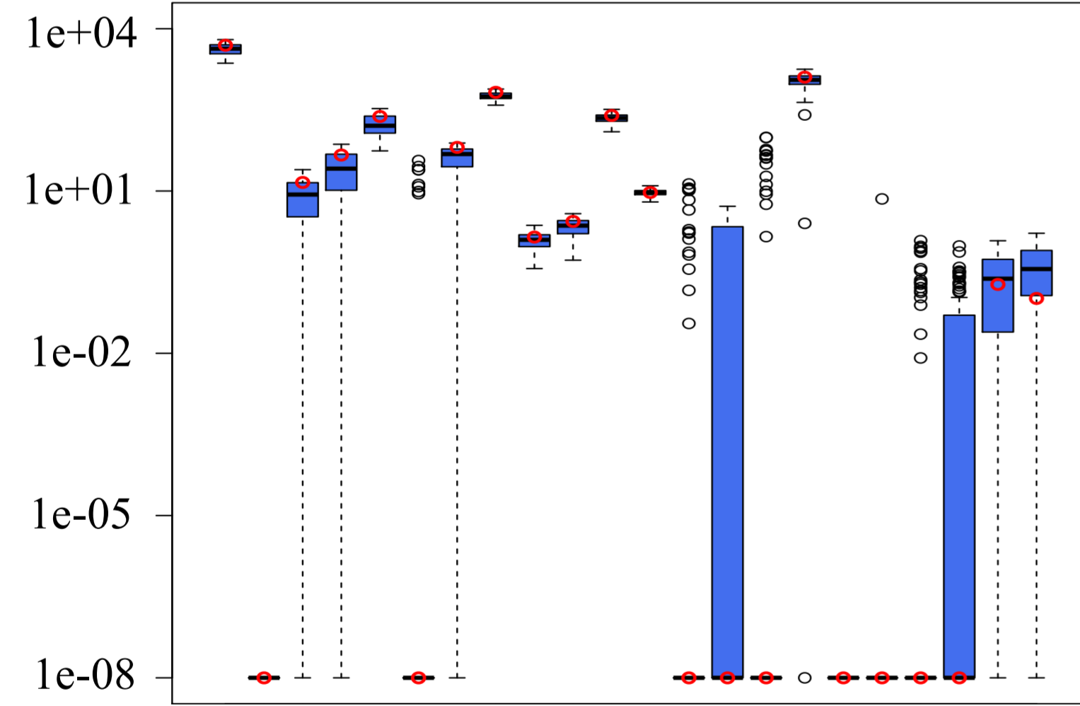
Construction works [ng m -3 ]
