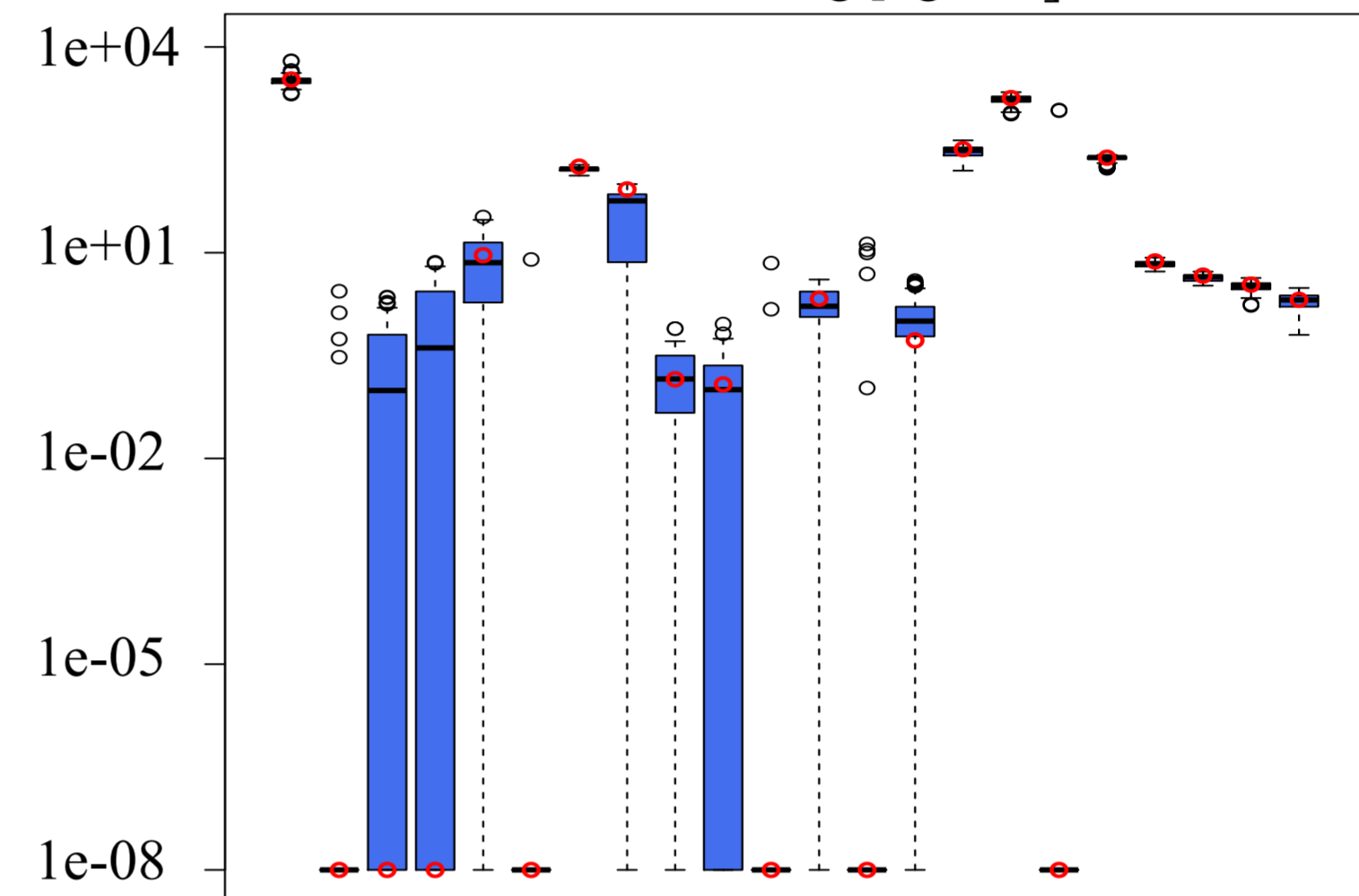
Biomass burning [ng m -3 ]
