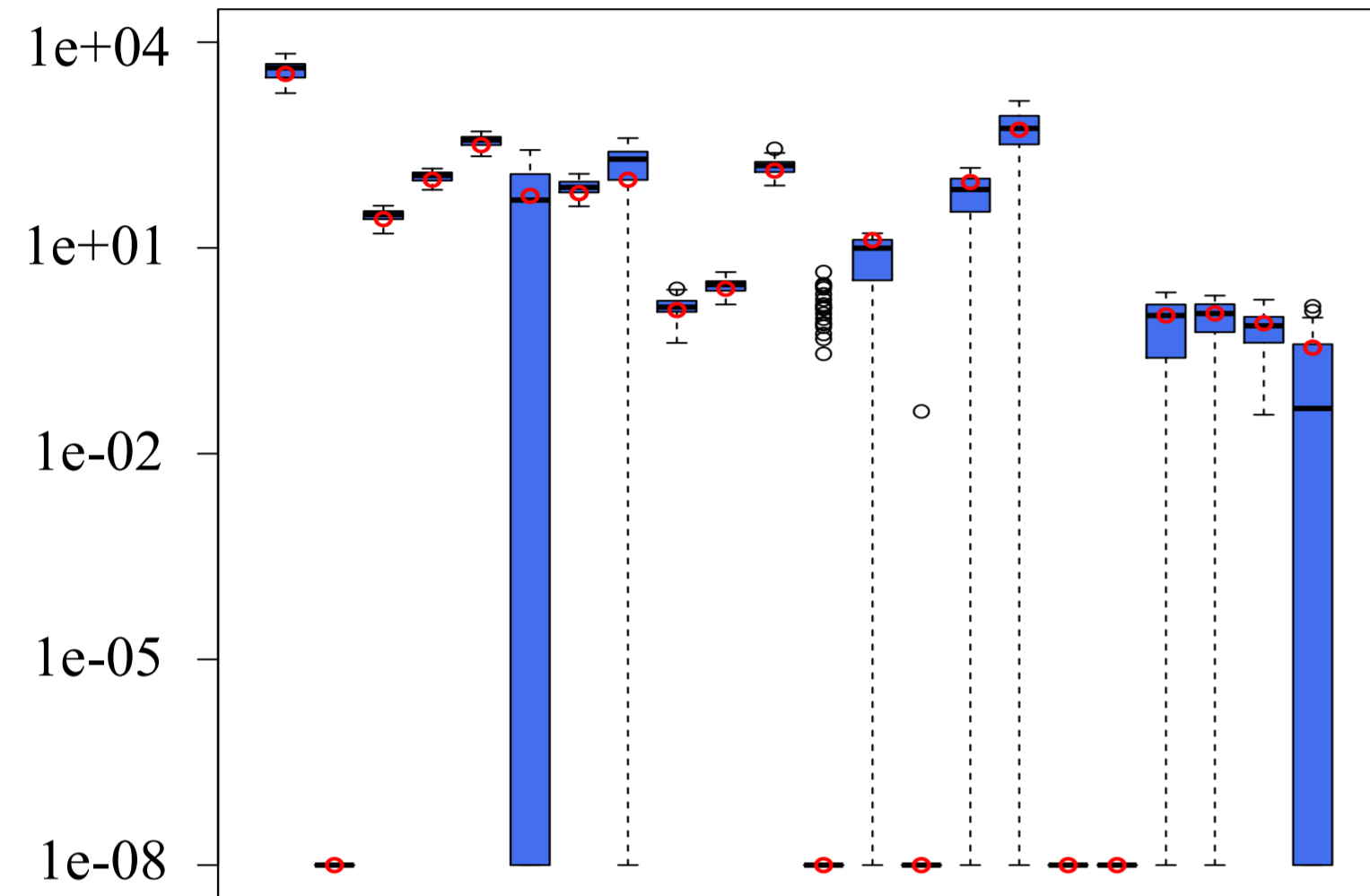
Resuspended dust [ng m -3 ]
