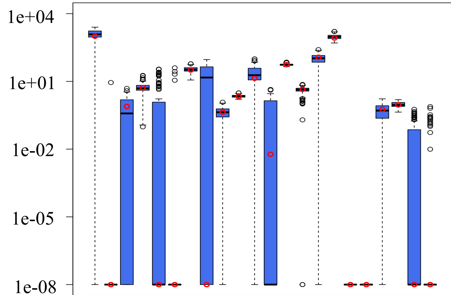
Industry [ng m -3 ]
