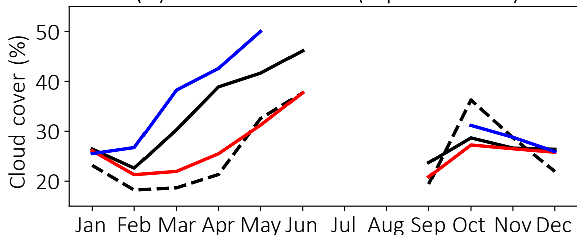
(f) Snow covered (ice clouds)
