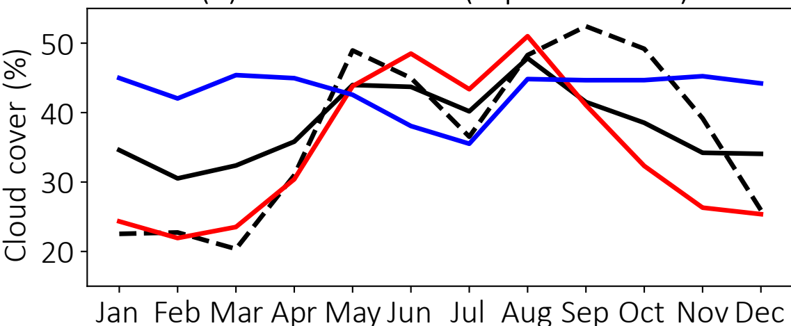
(e) Ice covered (ice clouds)
