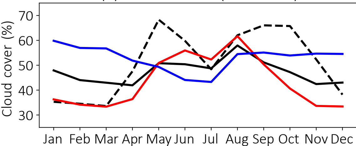
(c) Ice covered (liquid clouds)
