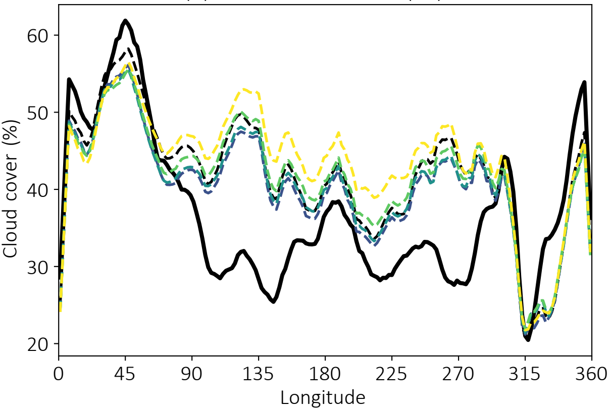
(a) Low-level clouds (all)
