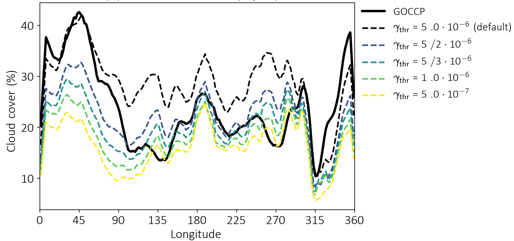
(b) Low-level clouds (liquid)
