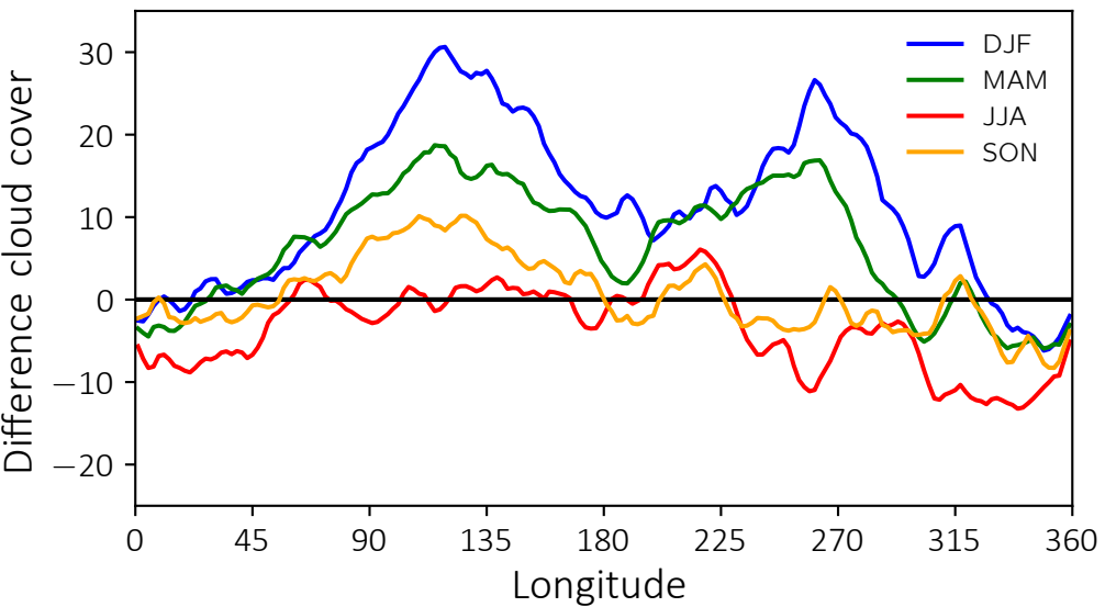
Total clouds
