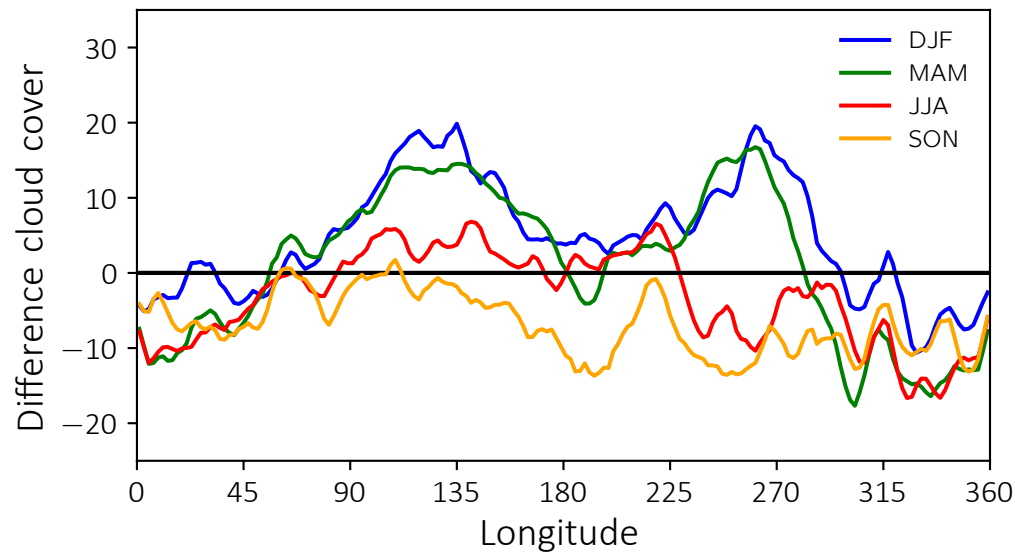
Low clouds
