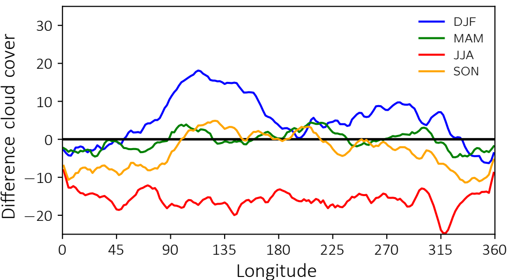
Mid clouds
