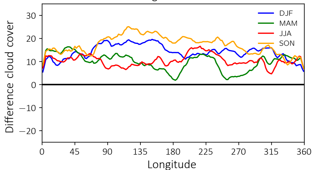
High clouds
