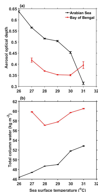
Figure 6. (a) Mean and standard error of AOD and (b) TCW (in kg m -2 ) with SST over the AS and the BOB during ISM.
