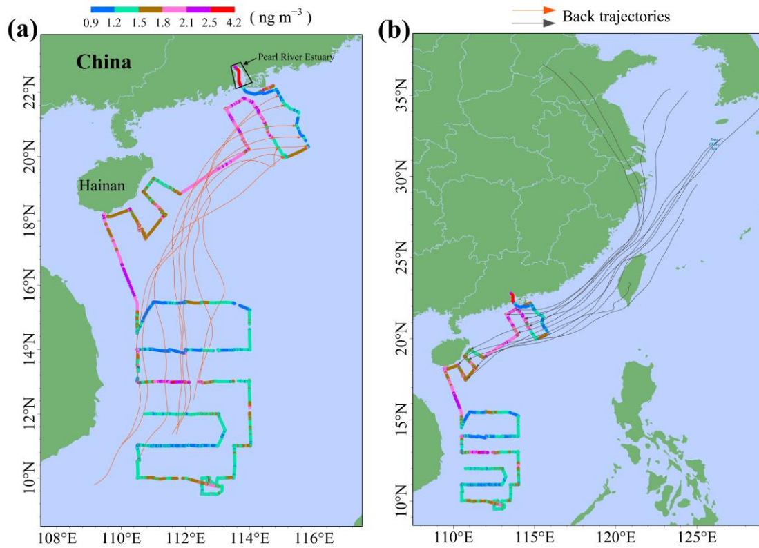
61 Figure S2. GEM concentrations over the northern SCS and 72-h back-trajectories arriving at some stations.
