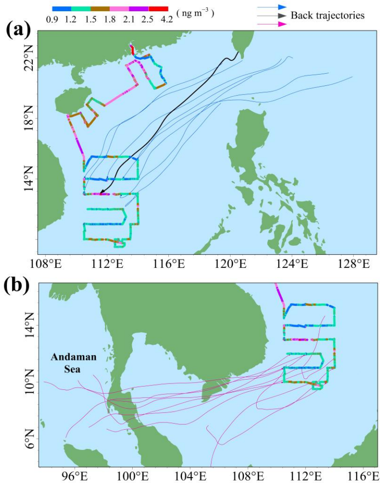
63 Figure S3. GEM concentrations over the western SCS and 72-h back-trajectories arriving at some stations.
