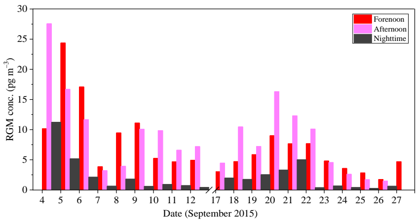
66 Figure S4. RGM concentrations in forenoon, afternoon and nighttime.
