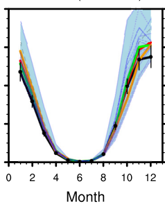
Palmer (64.77° S)
