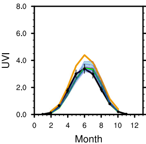
Barrow (72.32° N)
