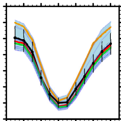
Lauder (45.04° S)
