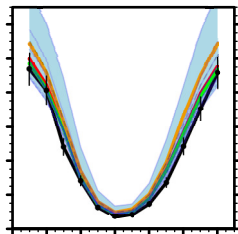
Palmer (64.77° S)
