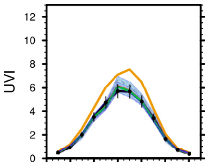
Barrow (72.32° N)
